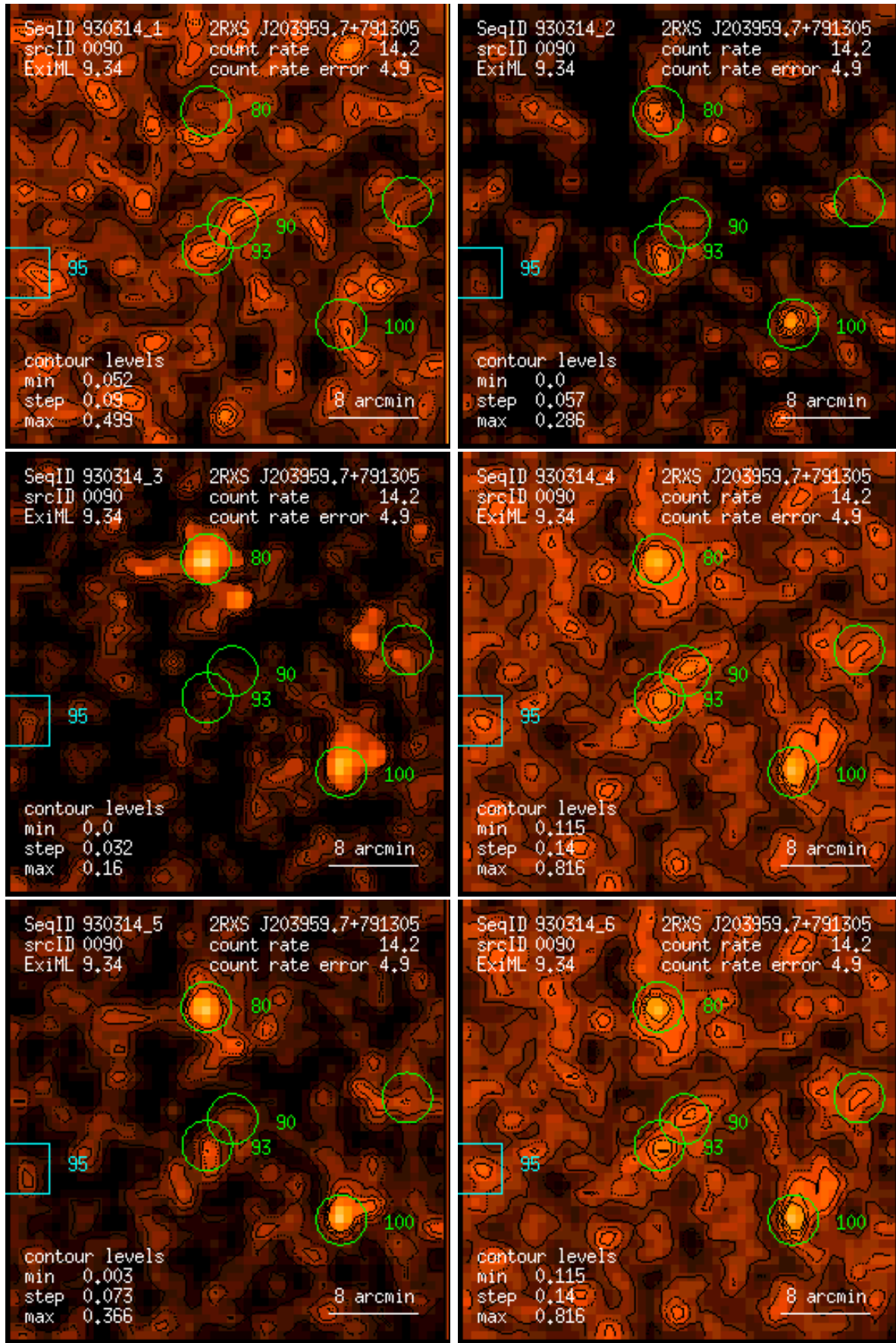
Figure 90: RASS 930314: detection 0090: band rate images, Gaussian filter: (1) PSPC channels 11 – 41, (2) 52 – 90, (3) 91 – 201, (4) 11 – 235, (5) 52 – 201, (6) 11 – 201. Broad band rates in counts/ks. Band rate contour levels in counts/ks/arcmin 2 .
