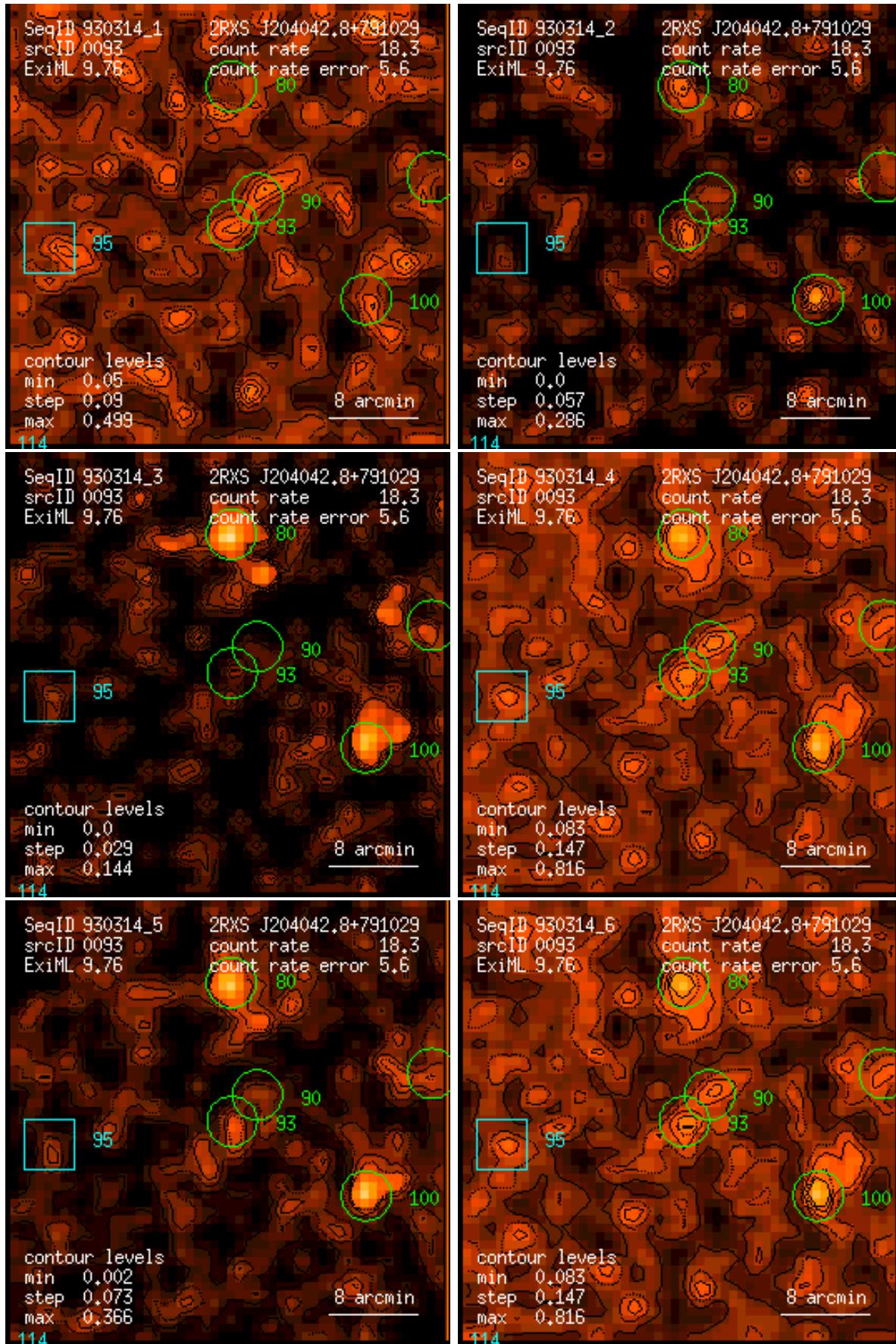
Figure 93: RASS 930314: detection 0093: band rate images, Gaussian filter: (1) PSPC channels 11 – 41, (2) 52 – 90, (3) 91 – 201, (4) 11 – 235, (5) 52 – 201, (6) 11 – 201. Broad band rates in counts/ks. Band rate contour levels in counts/ks/arcmin 2 .
