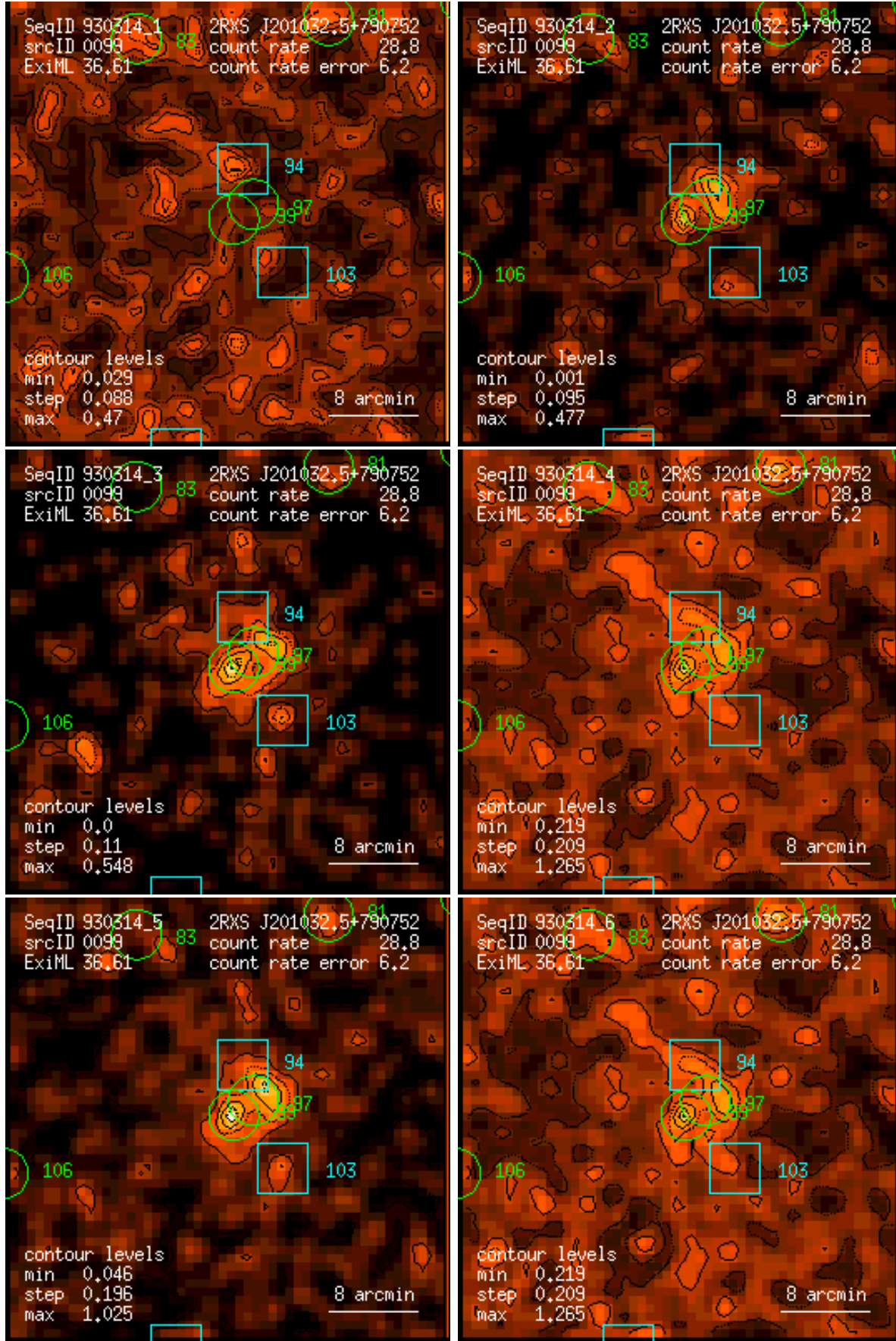
Figure 99: RASS 930314: detection 0099: band rate images, Gaussian filter: (1) PSPC channels 11 – 41, (2) 52 – 90, (3) 91 – 201, (4) 11 – 235, (5) 52 – 201, (6) 11 – 201. Broad band rates in counts/ks. Band rate contour levels in counts/ks/arcmin 2 .
