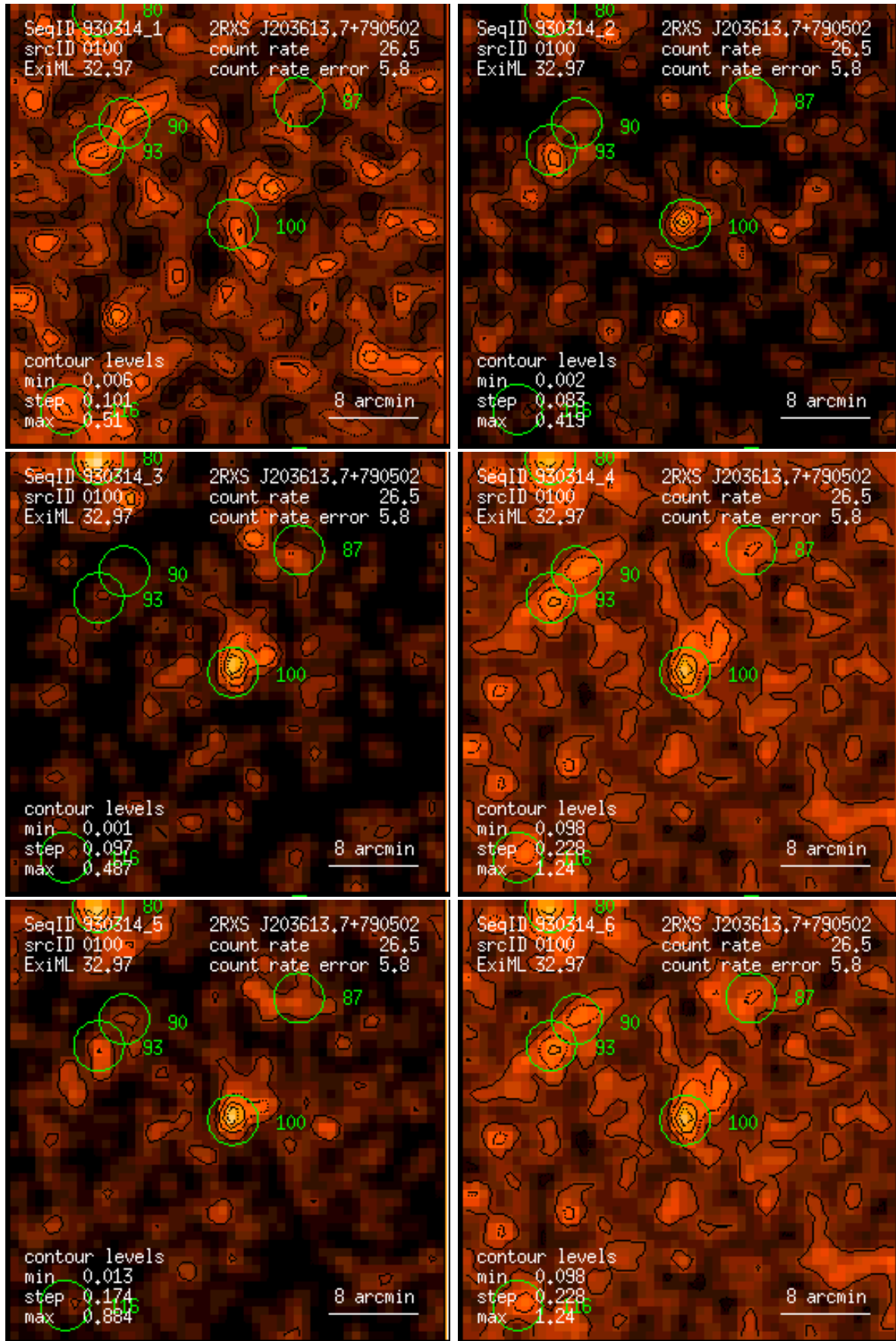
Figure 100: RASS 930314: detection 0100: band rate images, Gaussian filter: (1) PSPC channels 11 – 41, (2) 52 – 90, (3) 91 – 201, (4) 11 – 235, (5) 52 – 201, (6) 11 – 201. Broad band rates in counts/ks. Band rate contour levels in counts/ks/arcmin 2 .
