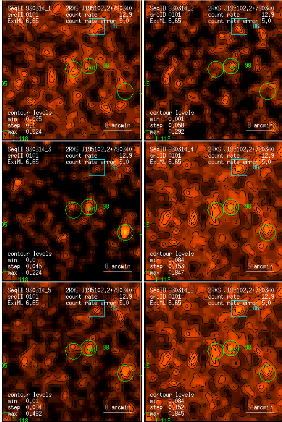
Figure 101: RASS 930314: detection 0101: band rate images, Gaussian filter: (1) PSPC channels 11 – 41, (2) 52 – 90, (3) 91 – 201, (4) 11 – 235, (5) 52 – 201, (6) 11 – 201. Broad band rates in counts/ks. Band rate contour levels in counts/ks/arcmin 2 .
