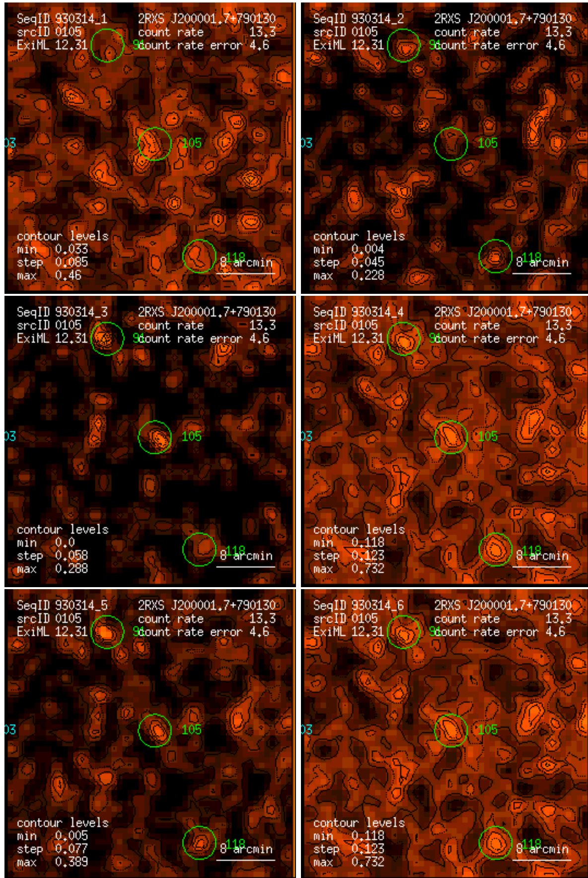
Figure 105: RASS 930314: detection 0105: band rate images, Gaussian filter: (1) PSPC channels 11 – 41, (2) 52 – 90, (3) 91 – 201, (4) 11 – 235, (5) 52 – 201, (6) 11 – 201. Broad band rates in counts/ks. Band rate contour levels in counts/ks/arcmin 2 .
