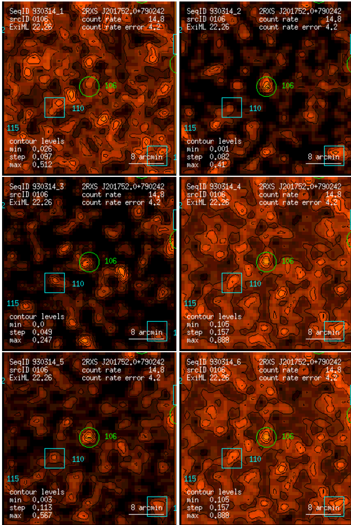
Figure 106: RASS 930314: detection 0106: band rate images, Gaussian filter: (1) PSPC channels 11 – 41, (2) 52 – 90, (3) 91 – 201, (4) 11 – 235, (5) 52 – 201, (6) 11 – 201. Broad band rates in counts/ks. Band rate contour levels in counts/ks/arcmin 2 .
