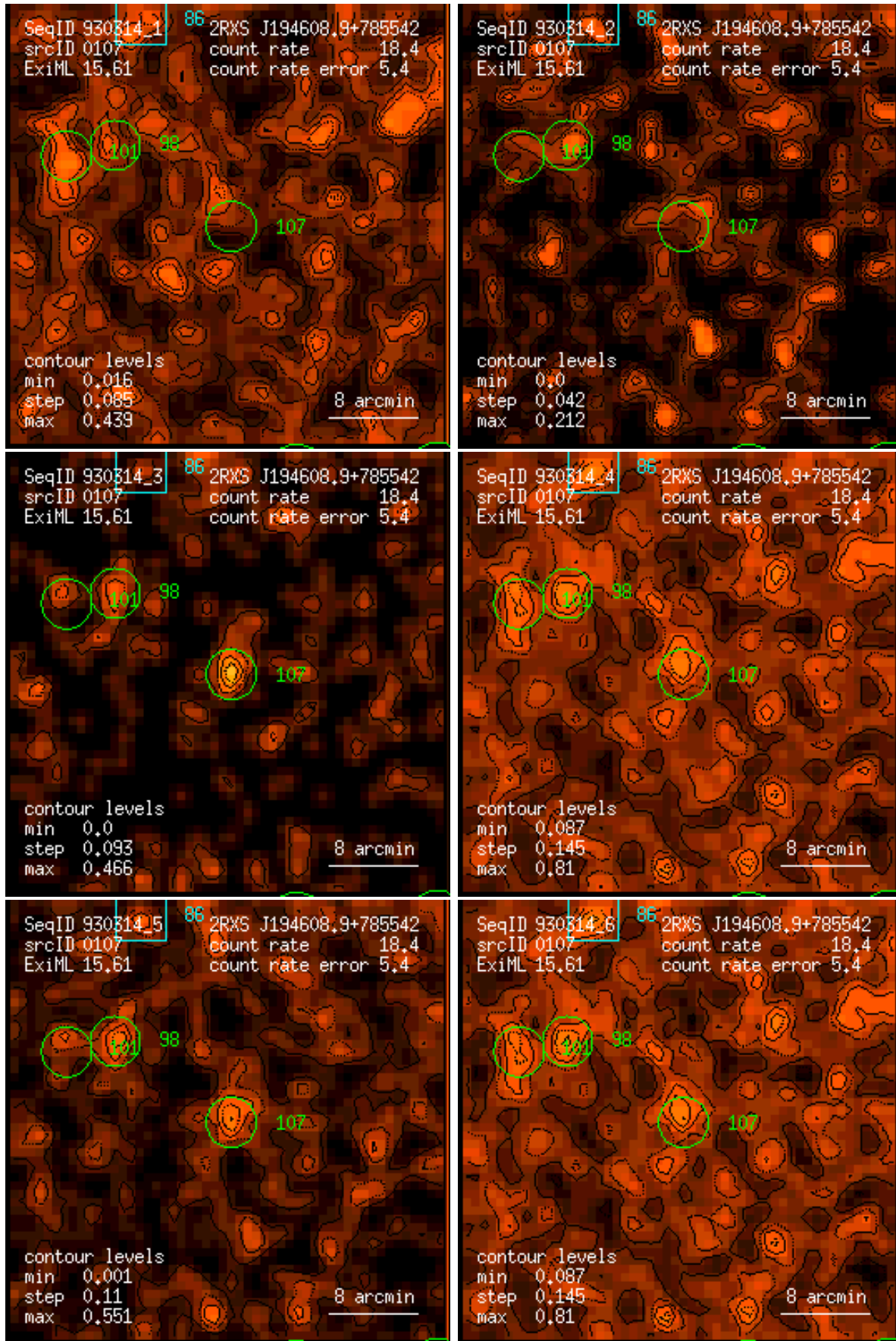
Figure 107: RASS 930314: detection 0107: band rate images, Gaussian filter: (1) PSPC channels 11 – 41, (2) 52 – 90, (3) 91 – 201, (4) 11 – 235, (5) 52 – 201, (6) 11 – 201. Broad band rates in counts/ks. Band rate contour levels in counts/ks/arcmin 2 .
