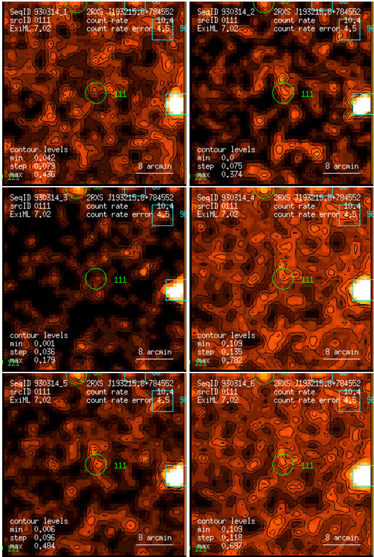
Figure 111: RASS 930314: detection 0111: band rate images, Gaussian filter: (1) PSPC channels 11 – 41, (2) 52 – 90, (3) 91 – 201, (4) 11 – 235, (5) 52 – 201, (6) 11 – 201. Broad band rates in counts/ks. Band rate contour levels in counts/ks/arcmin 2 .
