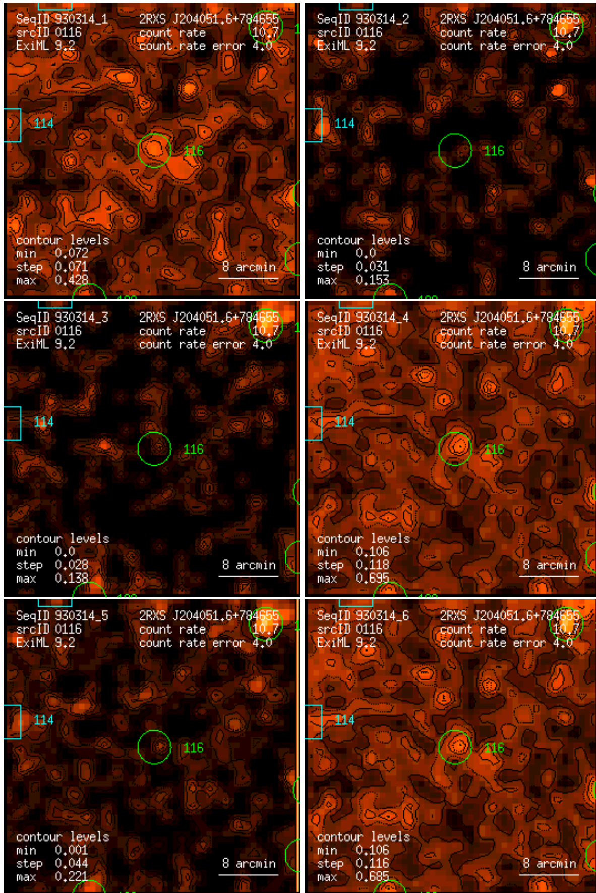
Figure 116: RASS 930314: detection 0116: band rate images, Gaussian filter: (1) PSPC channels 11 – 41, (2) 52 – 90, (3) 91 – 201, (4) 11 – 235, (5) 52 – 201, (6) 11 – 201. Broad band rates in counts/ks. Band rate contour levels in counts/ks/arcmin 2 .
