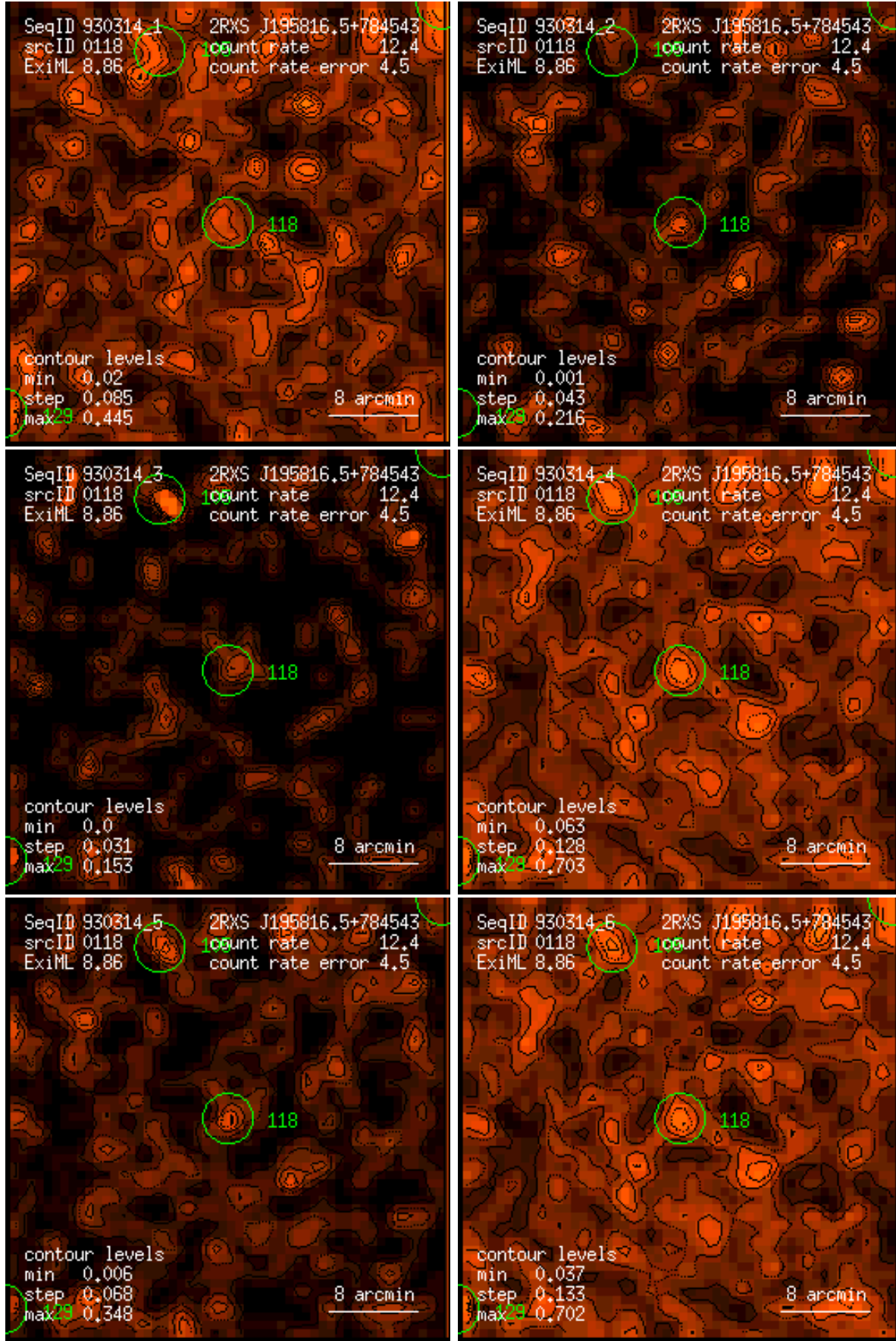
Figure 118: RASS 930314: detection 0118: band rate images, Gaussian filter: (1) PSPC channels 11 – 41, (2) 52 – 90, (3) 91 – 201, (4) 11 – 235, (5) 52 – 201, (6) 11 – 201. Broad band rates in counts/ks. Band rate contour levels in counts/ks/arcmin 2 .
