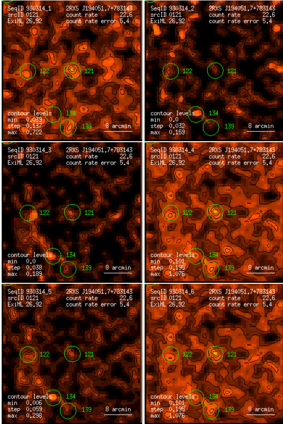
Figure 121: RASS 930314: detection 0121: band rate images, Gaussian filter: (1) PSPC channels 11 – 41, (2) 52 – 90, (3) 91 – 201, (4) 11 – 235, (5) 52 – 201, (6) 11 – 201. Broad band rates in counts/ks. Band rate contour levels in counts/ks/arcmin 2 .
