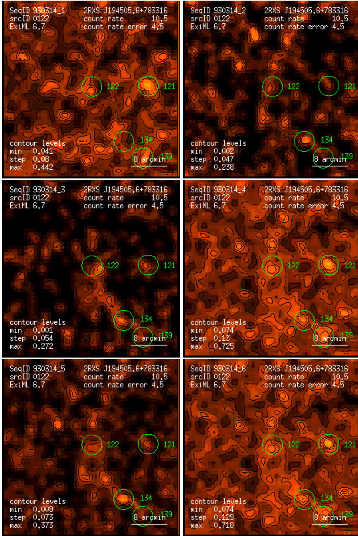
Figure 122: RASS 930314: detection 0122: band rate images, Gaussian filter: (1) PSPC channels 11 – 41, (2) 52 – 90, (3) 91 – 201, (4) 11 – 235, (5) 52 – 201, (6) 11 – 201. Broad band rates in counts/ks. Band rate contour levels in counts/ks/arcmin 2 .
