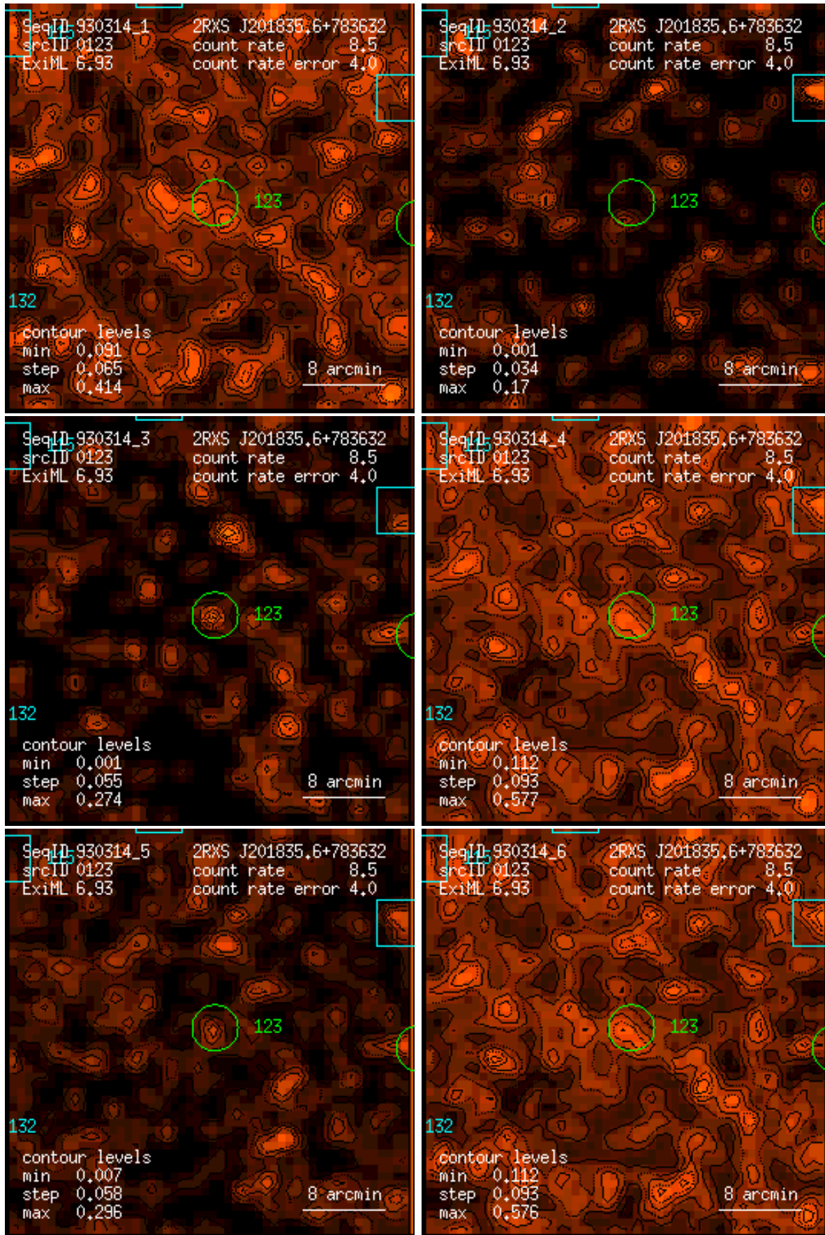
Figure 123: RASS 930314: detection 0123: band rate images, Gaussian filter: (1) PSPC channels 11 – 41, (2) 52 – 90, (3) 91 – 201, (4) 11 – 235, (5) 52 – 201, (6) 11 – 201. Broad band rates in counts/ks. Band rate contour levels in counts/ks/arcmin 2 .
