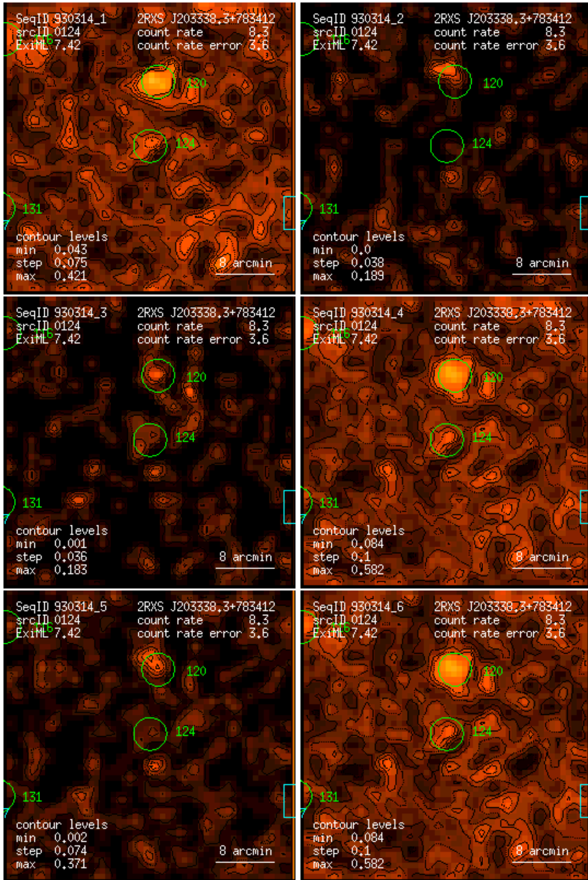
Figure 124: RASS 930314: detection 0124: band rate images, Gaussian filter: (1) PSPC channels 11 – 41, (2) 52 – 90, (3) 91 – 201, (4) 11 – 235, (5) 52 – 201, (6) 11 – 201. Broad band rates in counts/ks. Band rate contour levels in counts/ks/arcmin 2 .
