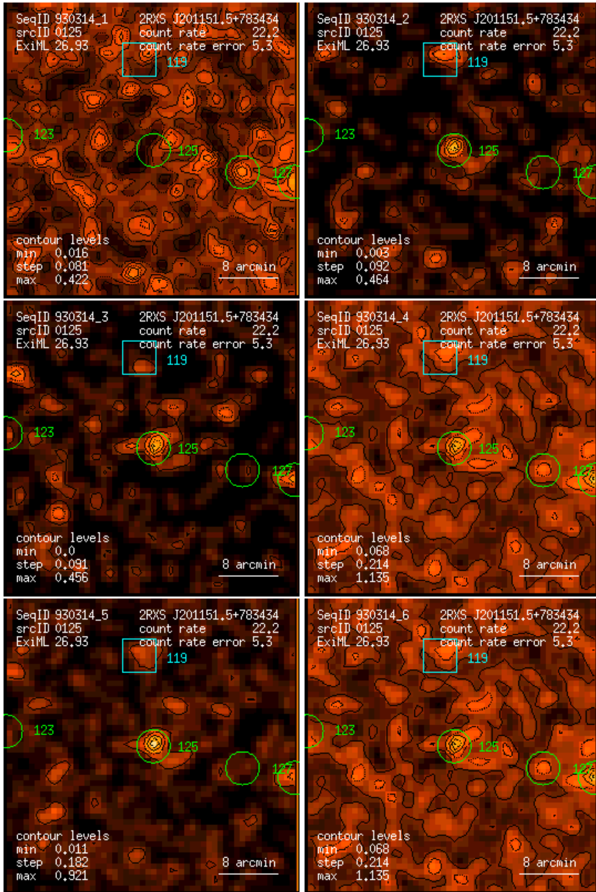
Figure 125: RASS 930314: detection 0125: band rate images, Gaussian filter: (1) PSPC channels 11 – 41, (2) 52 – 90, (3) 91 – 201, (4) 11 – 235, (5) 52 – 201, (6) 11 – 201. Broad band rates in counts/ks. Band rate contour levels in counts/ks/arcmin 2 .
