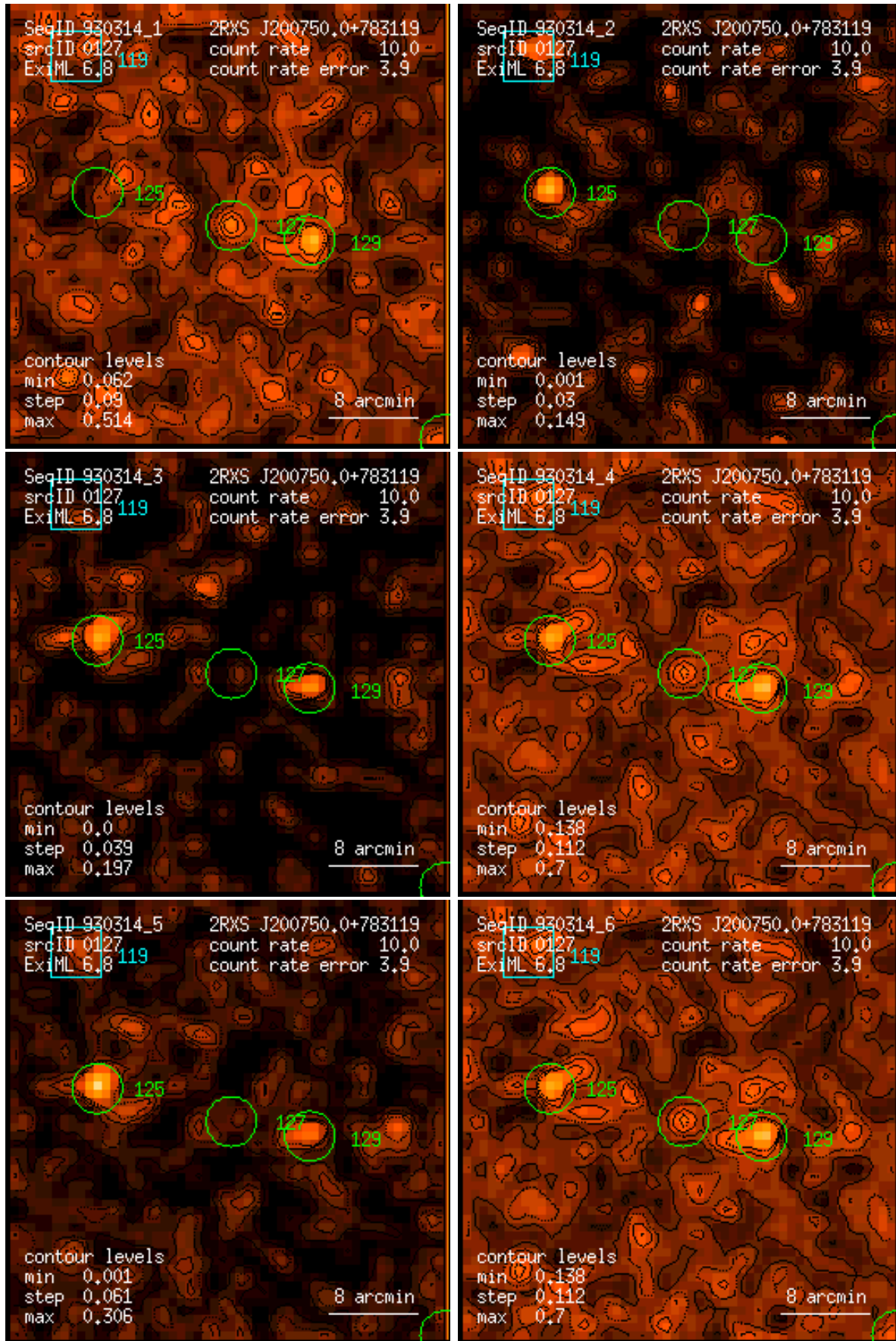
Figure 127: RASS 930314: detection 0127: band rate images, Gaussian filter: (1) PSPC channels 11 – 41, (2) 52 – 90, (3) 91 – 201, (4) 11 – 235, (5) 52 – 201, (6) 11 – 201. Broad band rates in counts/ks. Band rate contour levels in counts/ks/arcmin 2 .
