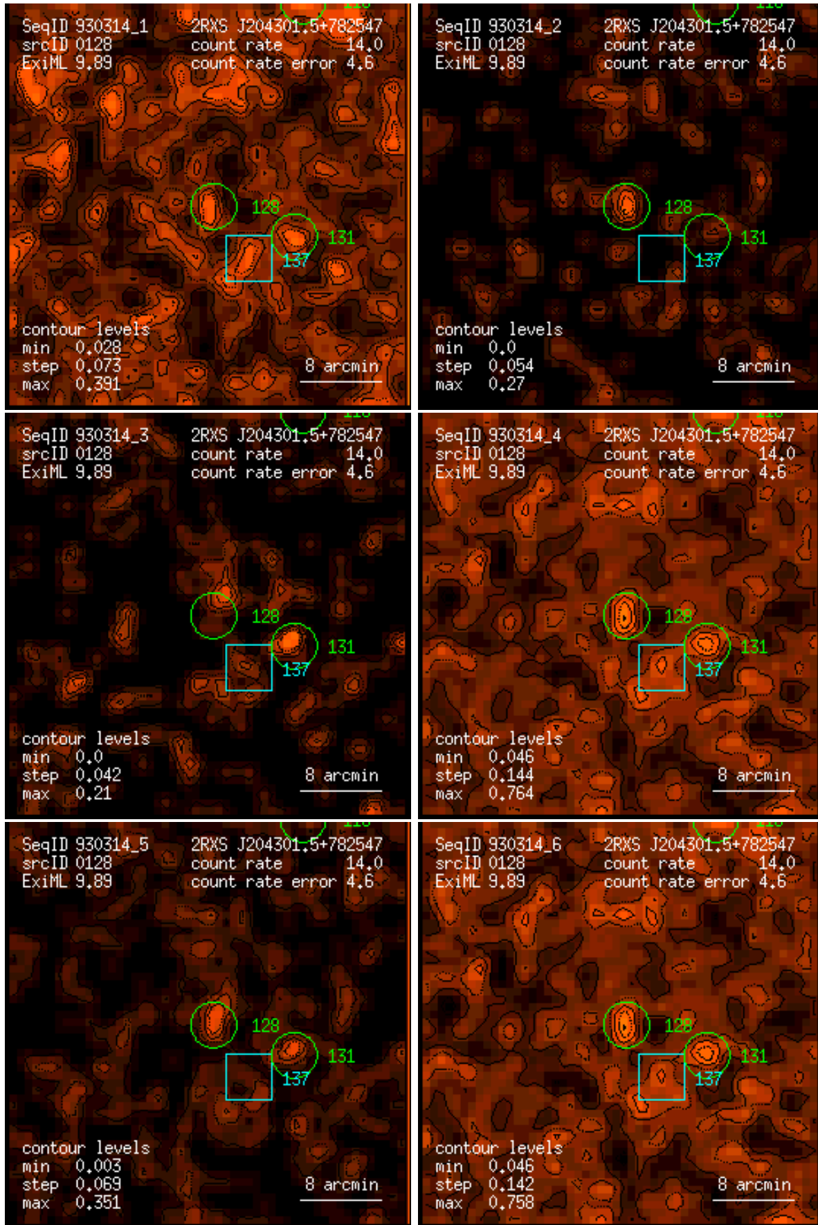
Figure 128: RASS 930314: detection 0128: band rate images, Gaussian filter: (1) PSPC channels 11 – 41, (2) 52 – 90, (3) 91 – 201, (4) 11 – 235, (5) 52 – 201, (6) 11 – 201. Broad band rates in counts/ks. Band rate contour levels in counts/ks/arcmin 2 .
