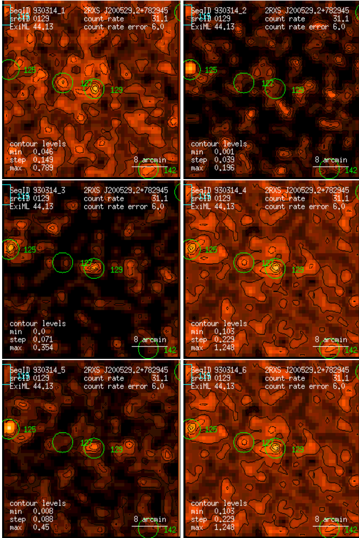
Figure 129: RASS 930314: detection 0129: band rate images, Gaussian filter: (1) PSPC channels 11 – 41, (2) 52 – 90, (3) 91 – 201, (4) 11 – 235, (5) 52 – 201, (6) 11 – 201. Broad band rates in counts/ks. Band rate contour levels in counts/ks/arcmin 2 .
