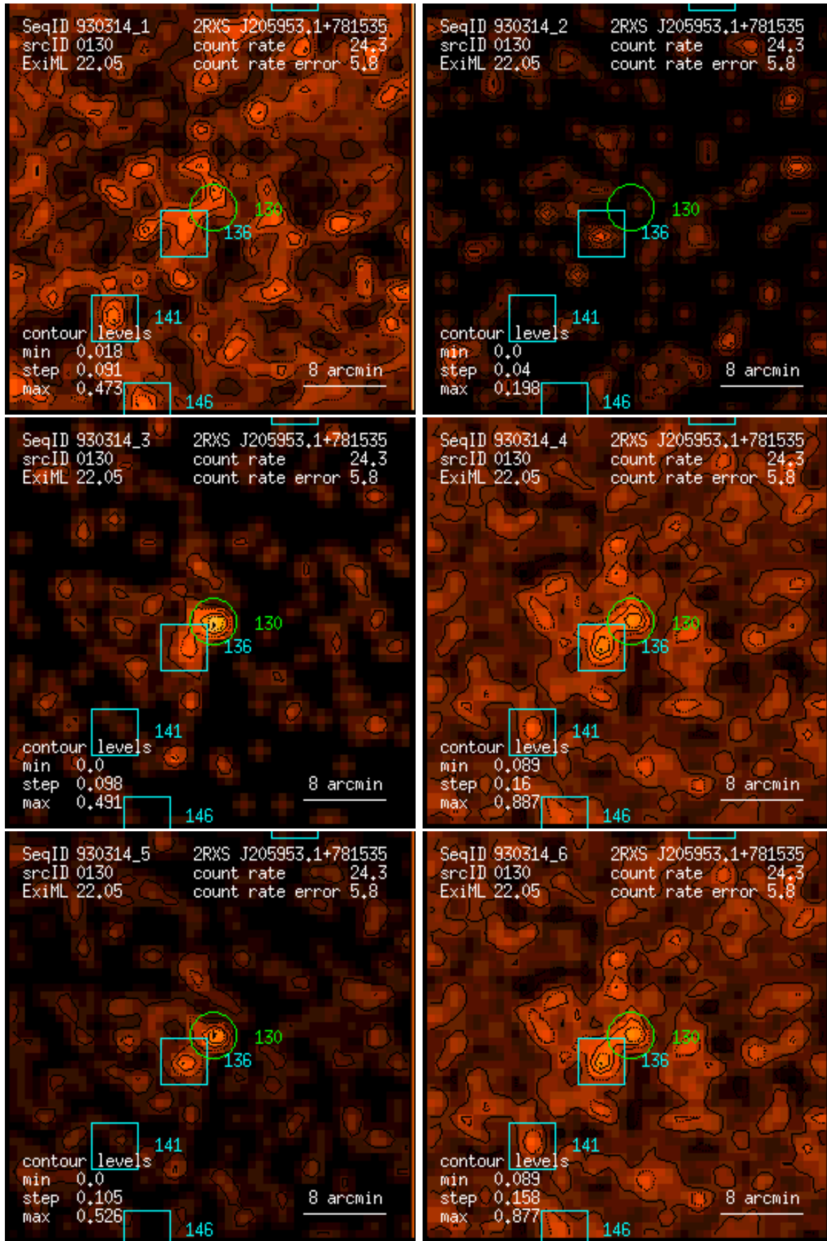
Figure 130: RASS 930314: detection 0130: band rate images, Gaussian filter: (1) PSPC channels 11 – 41, (2) 52 – 90, (3) 91 – 201, (4) 11 – 235, (5) 52 – 201, (6) 11 – 201. Broad band rates in counts/ks. Band rate contour levels in counts/ks/arcmin 2 .
