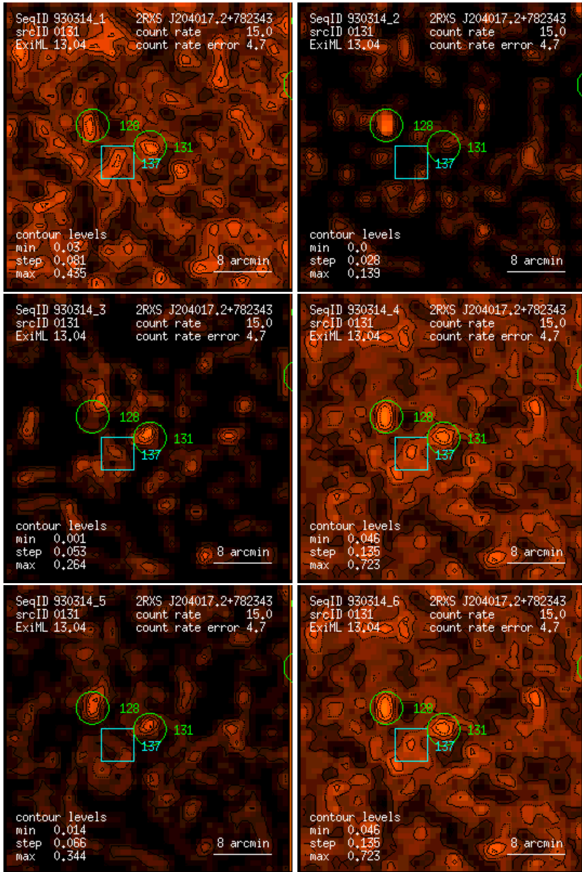
Figure 131: RASS 930314: detection 0131: band rate images, Gaussian filter: (1) PSPC channels 11 – 41, (2) 52 – 90, (3) 91 – 201, (4) 11 – 235, (5) 52 – 201, (6) 11 – 201. Broad band rates in counts/ks. Band rate contour levels in counts/ks/arcmin 2 .
