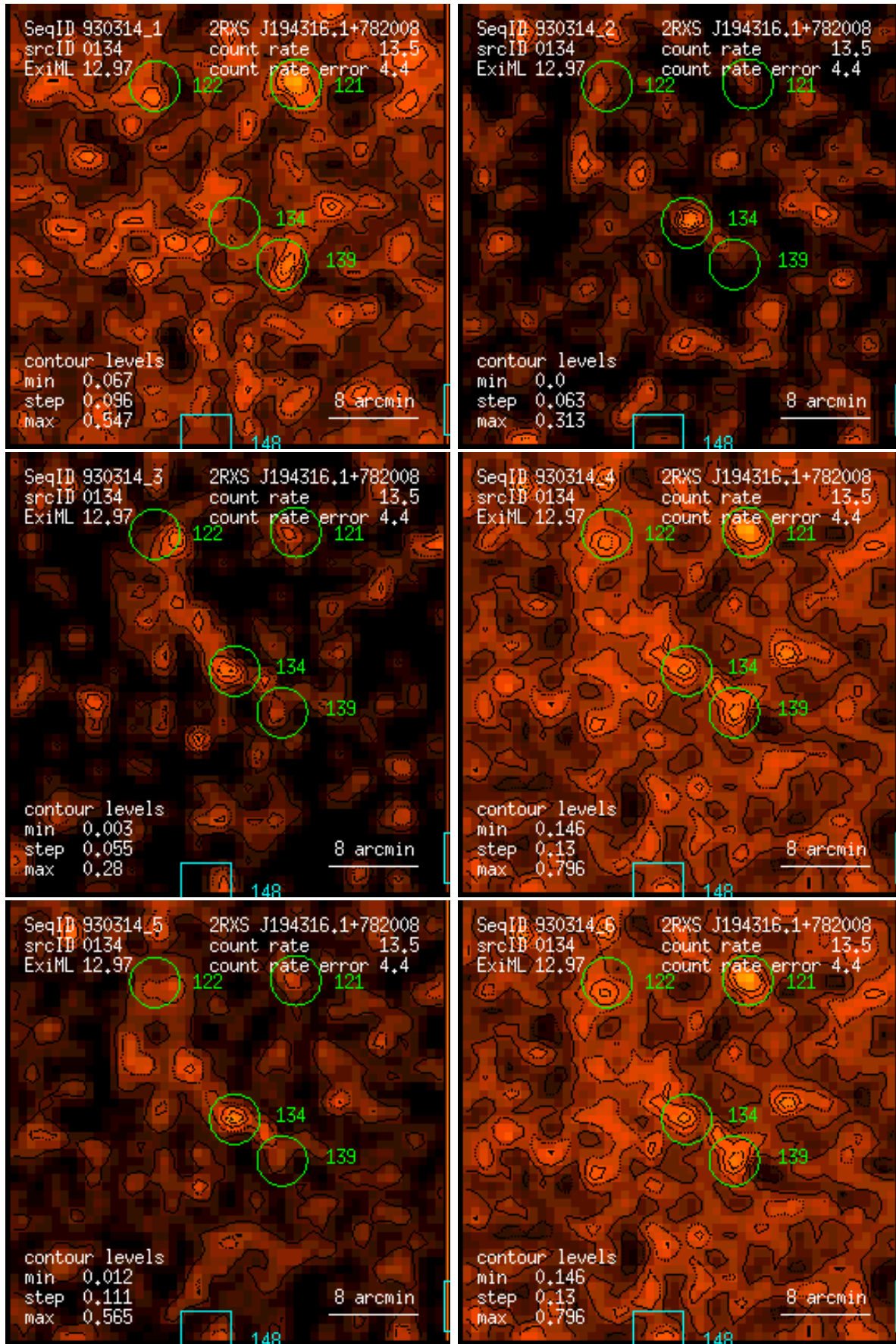
Figure 134: RASS 930314: detection 0134: band rate images, Gaussian filter: (1) PSPC channels 11 – 41, (2) 52 – 90, (3) 91 – 201, (4) 11 – 235, (5) 52 – 201, (6) 11 – 201. Broad band rates in counts/ks. Band rate contour levels in counts/ks/arcmin 2 .
