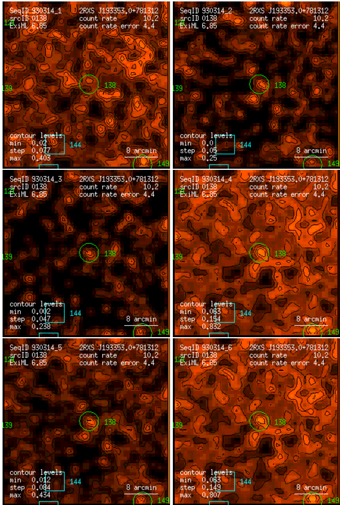
Figure 138: RASS 930314: detection 0138: band rate images, Gaussian filter: (1) PSPC channels 11 – 41, (2) 52 – 90, (3) 91 – 201, (4) 11 – 235, (5) 52 – 201, (6) 11 – 201. Broad band rates in counts/ks. Band rate contour levels in counts/ks/arcmin 2 .
