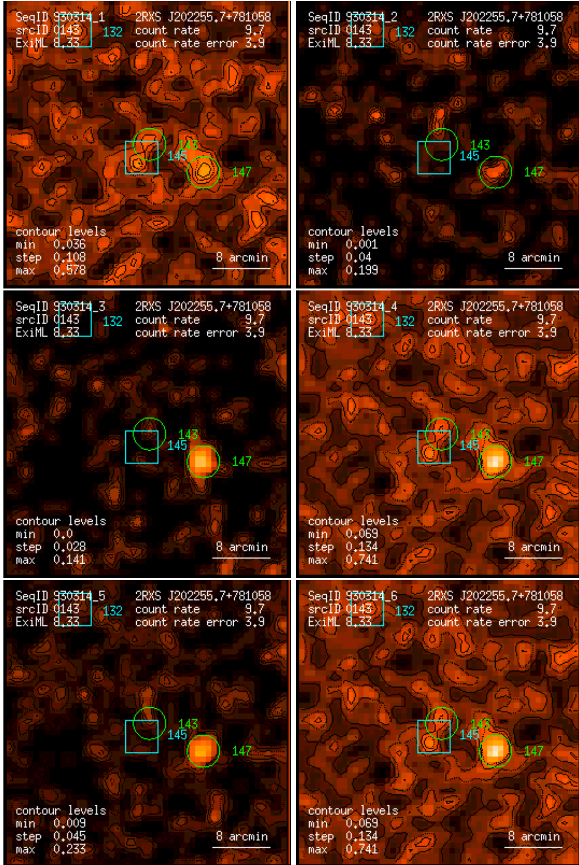
Figure 143: RASS 930314: detection 0143: band rate images, Gaussian filter: (1) PSPC channels 11 – 41, (2) 52 – 90, (3) 91 – 201, (4) 11 – 235, (5) 52 – 201, (6) 11 – 201. Broad band rates in counts/ks. Band rate contour levels in counts/ks/arcmin 2 .
