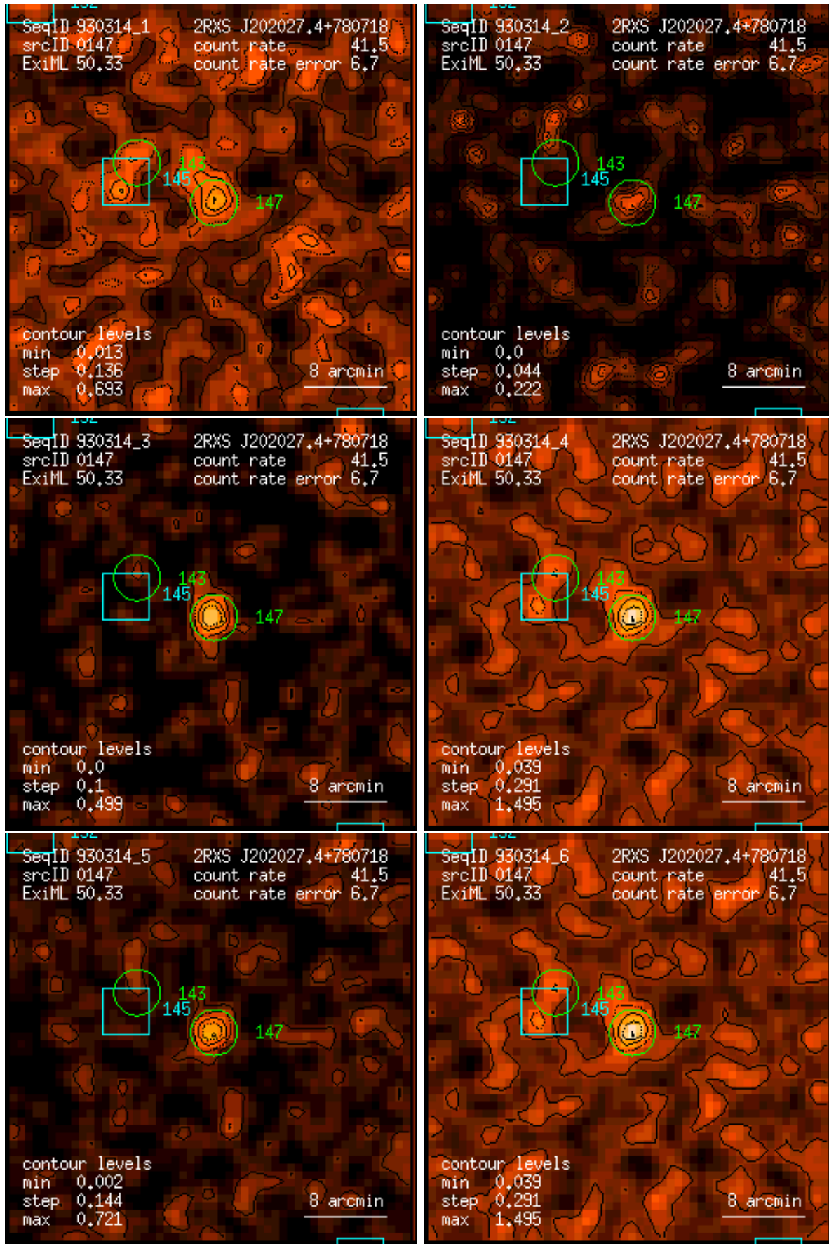
Figure 147: RASS 930314: detection 0147: band rate images, Gaussian filter: (1) PSPC channels 11 – 41, (2) 52 – 90, (3) 91 – 201, (4) 11 – 235, (5) 52 – 201, (6) 11 – 201. Broad band rates in counts/ks. Band rate contour levels in counts/ks/arcmin 2 .
