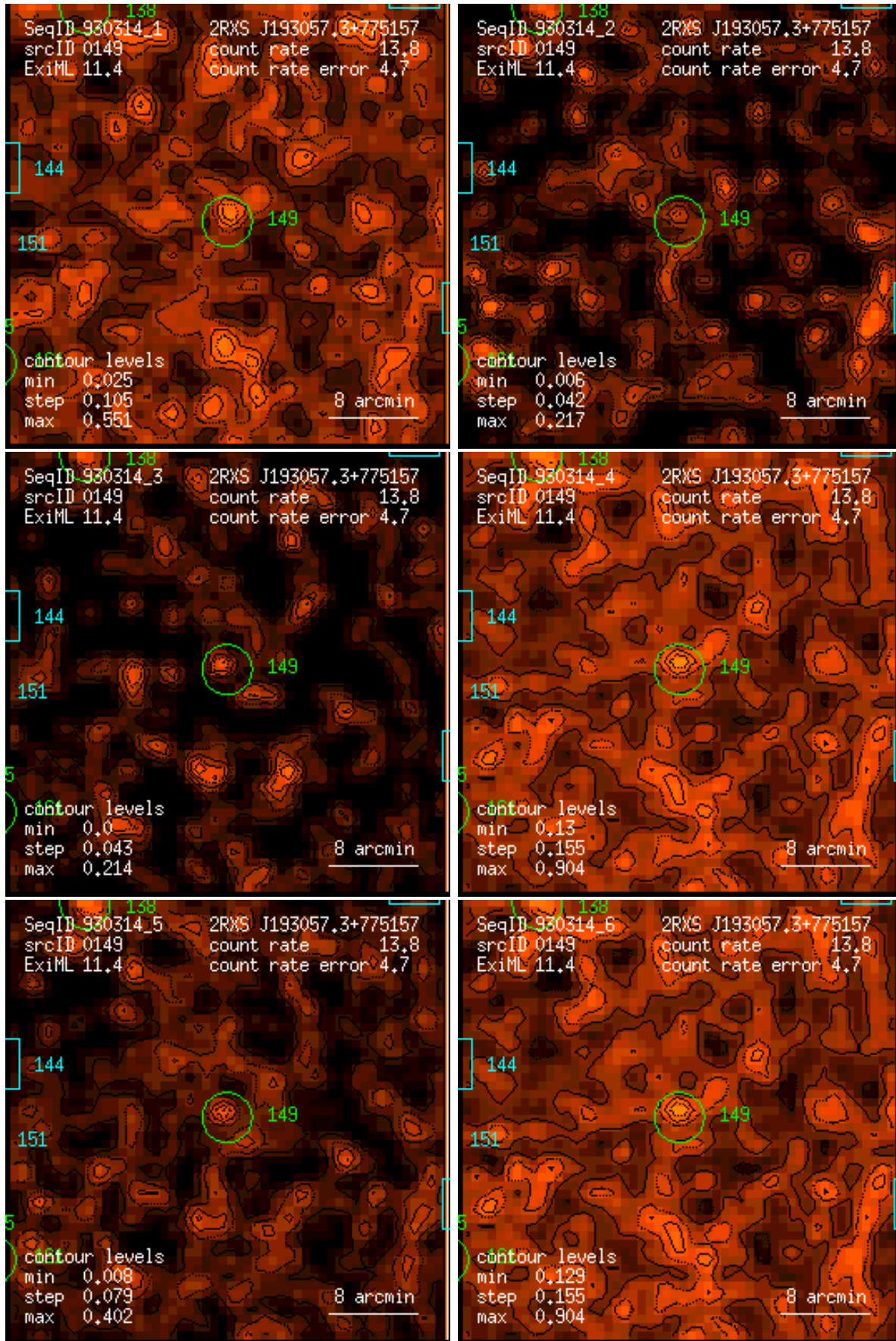
Figure 149: RASS 930314: detection 0149: band rate images, Gaussian filter: (1) PSPC channels 11 – 41, (2) 52 – 90, (3) 91 – 201, (4) 11 – 235, (5) 52 – 201, (6) 11 – 201. Broad band rates in counts/ks. Band rate contour levels in counts/ks/arcmin 2 .
