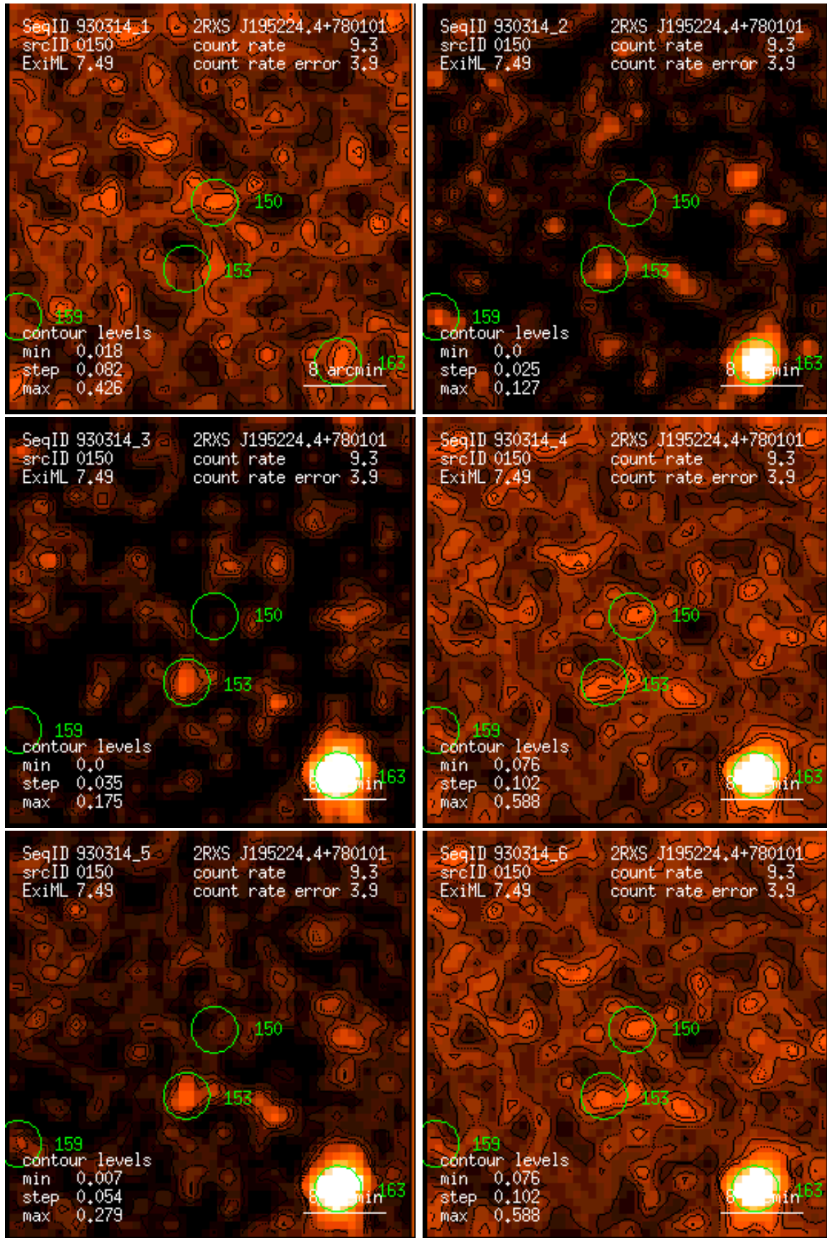
Figure 150: RASS 930314: detection 0150: band rate images, Gaussian filter: (1) PSPC channels 11 – 41, (2) 52 – 90, (3) 91 – 201, (4) 11 – 235, (5) 52 – 201, (6) 11 – 201. Broad band rates in counts/ks. Band rate contour levels in counts/ks/arcmin 2 .
