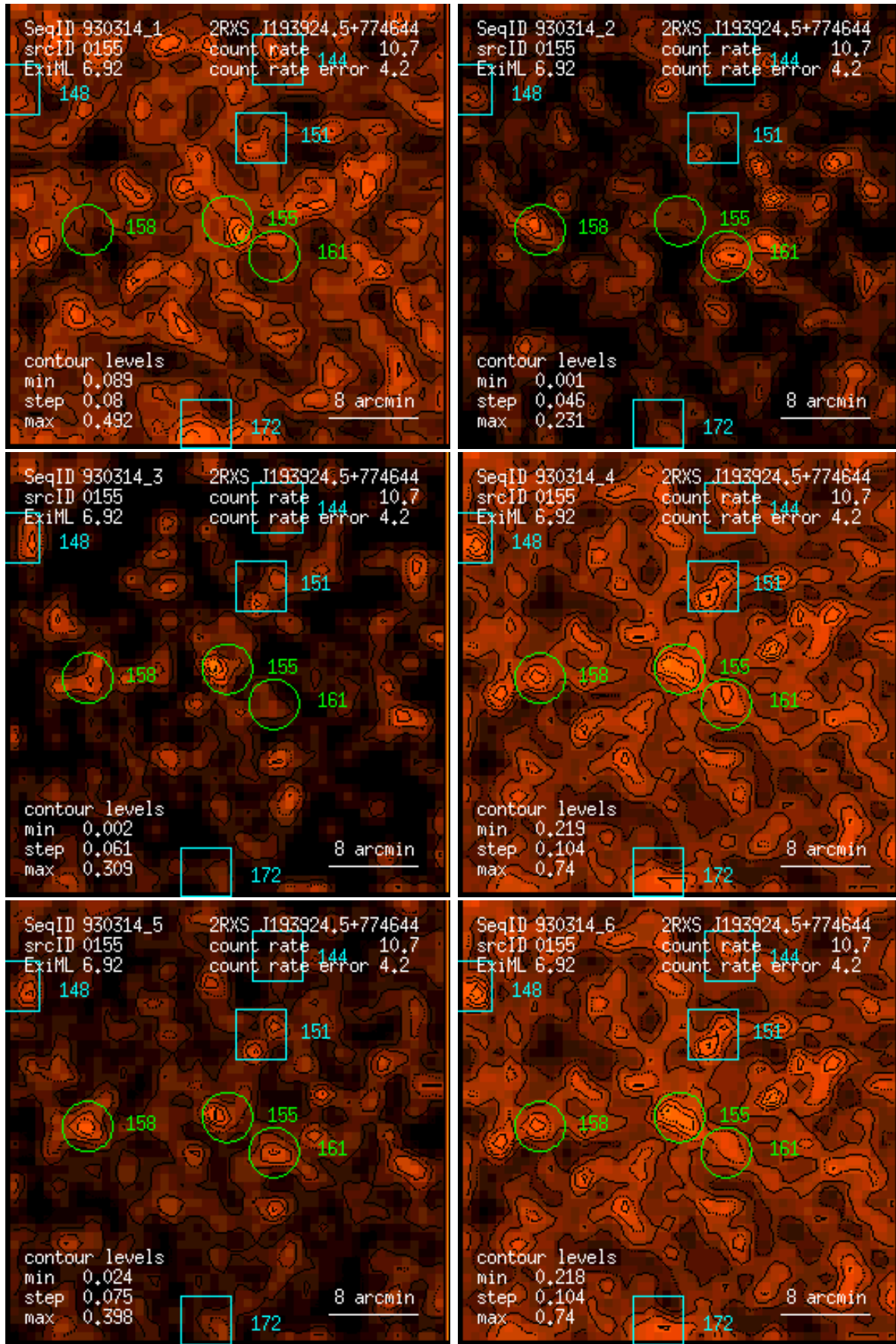
Figure 155: RASS 930314: detection 0155: band rate images, Gaussian filter: (1) PSPC channels 11 – 41, (2) 52 – 90, (3) 91 – 201, (4) 11 – 235, (5) 52 – 201, (6) 11 – 201. Broad band rates in counts/ks. Band rate contour levels in counts/ks/arcmin 2 .
