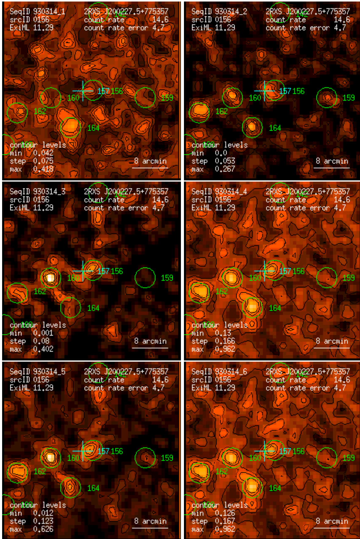
Figure 156: RASS 930314: detection 0156: band rate images, Gaussian filter: (1) PSPC channels 11 – 41, (2) 52 – 90, (3) 91 – 201, (4) 11 – 235, (5) 52 – 201, (6) 11 – 201. Broad band rates in counts/ks. Band rate contour levels in counts/ks/arcmin 2 .
