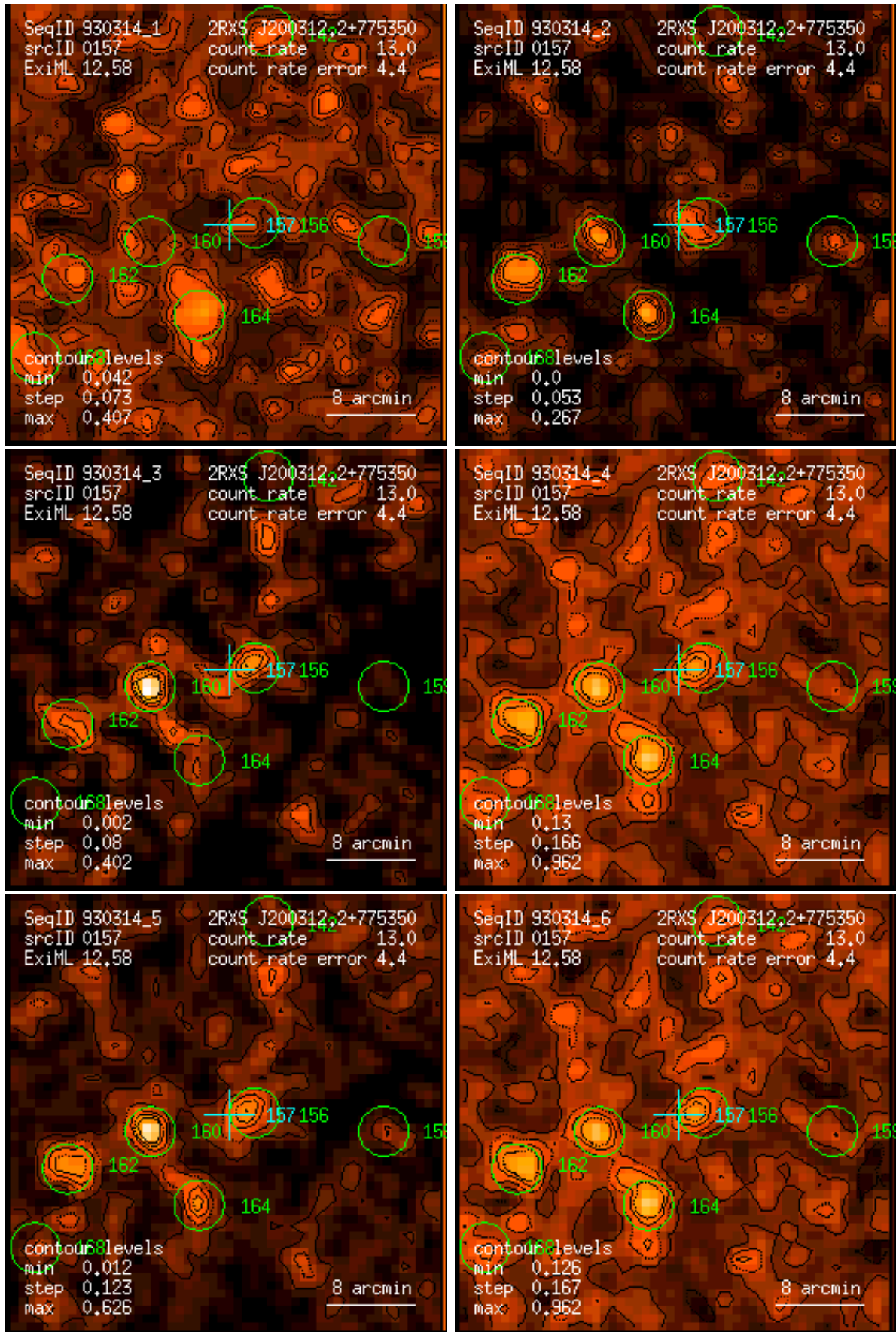
Figure 157: RASS 930314: detection 0157: band rate images, Gaussian filter: (1) PSPC channels 11 – 41, (2) 52 – 90, (3) 91 – 201, (4) 11 – 235, (5) 52 – 201, (6) 11 – 201. Broad band rates in counts/ks. Band rate contour levels in counts/ks/arcmin 2 .
