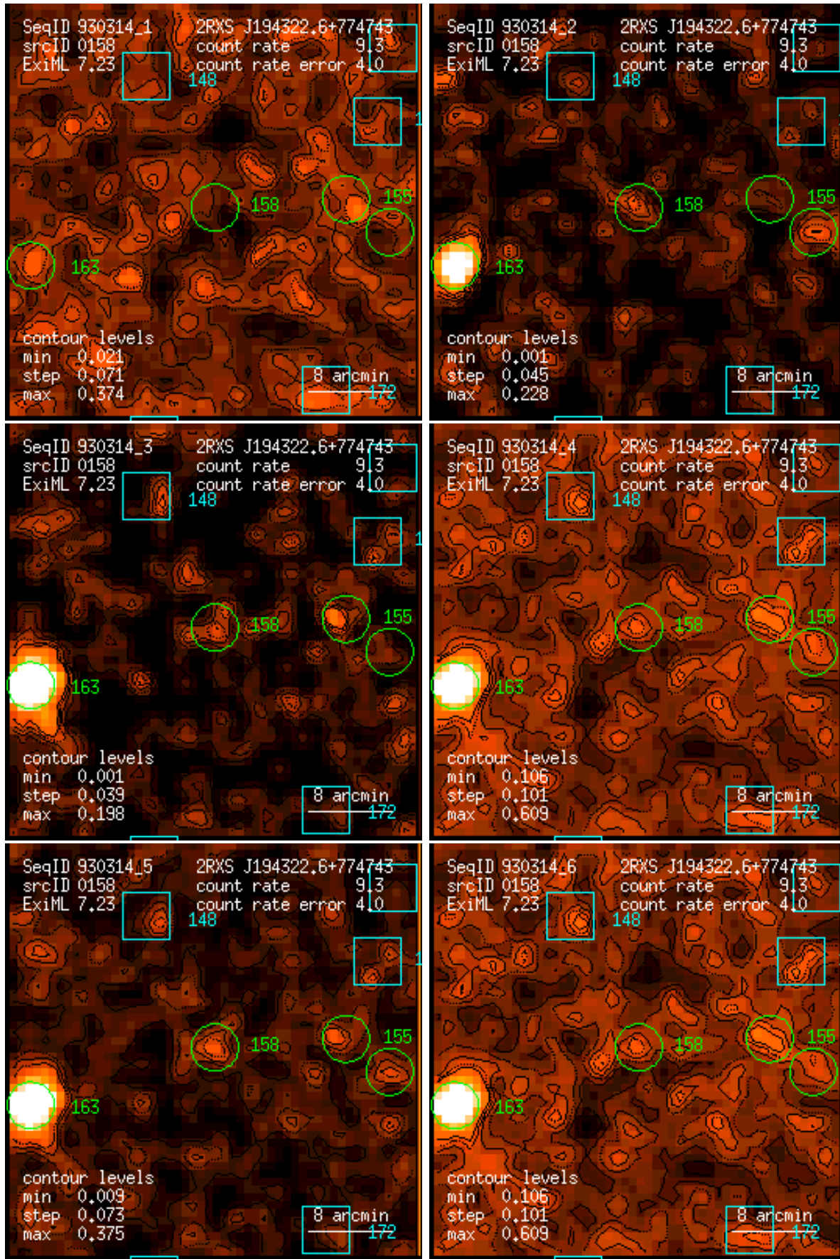
Figure 158: RASS 930314: detection 0158: band rate images, Gaussian filter: (1) PSPC channels 11 – 41, (2) 52 – 90, (3) 91 – 201, (4) 11 – 235, (5) 52 – 201, (6) 11 – 201. Broad band rates in counts/ks. Band rate contour levels in counts/ks/arcmin 2 .
