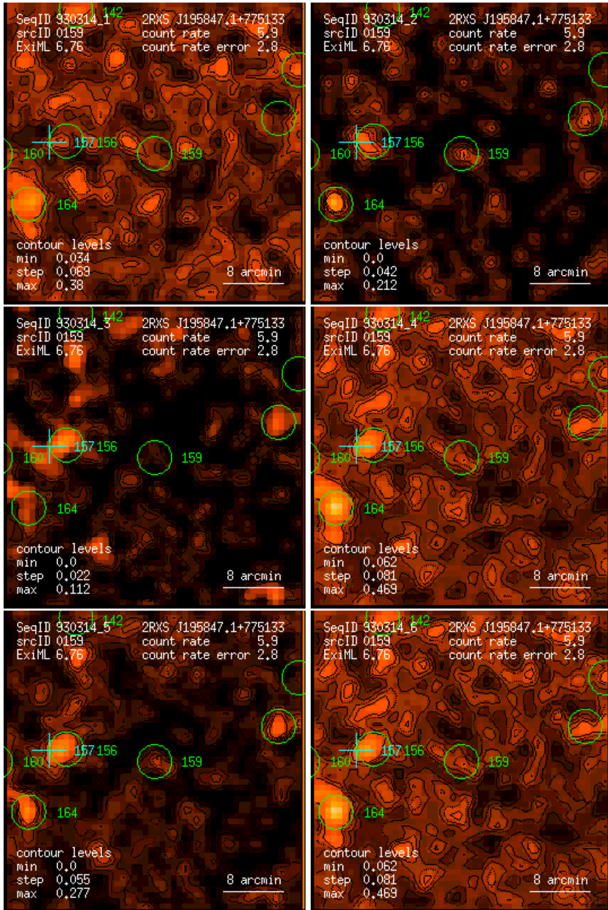
Figure 159: RASS 930314: detection 0159: band rate images, Gaussian filter: (1) PSPC channels 11 – 41, (2) 52 – 90, (3) 91 – 201, (4) 11 – 235, (5) 52 – 201, (6) 11 – 201. Broad band rates in counts/ks. Band rate contour levels in counts/ks/arcmin 2 .
