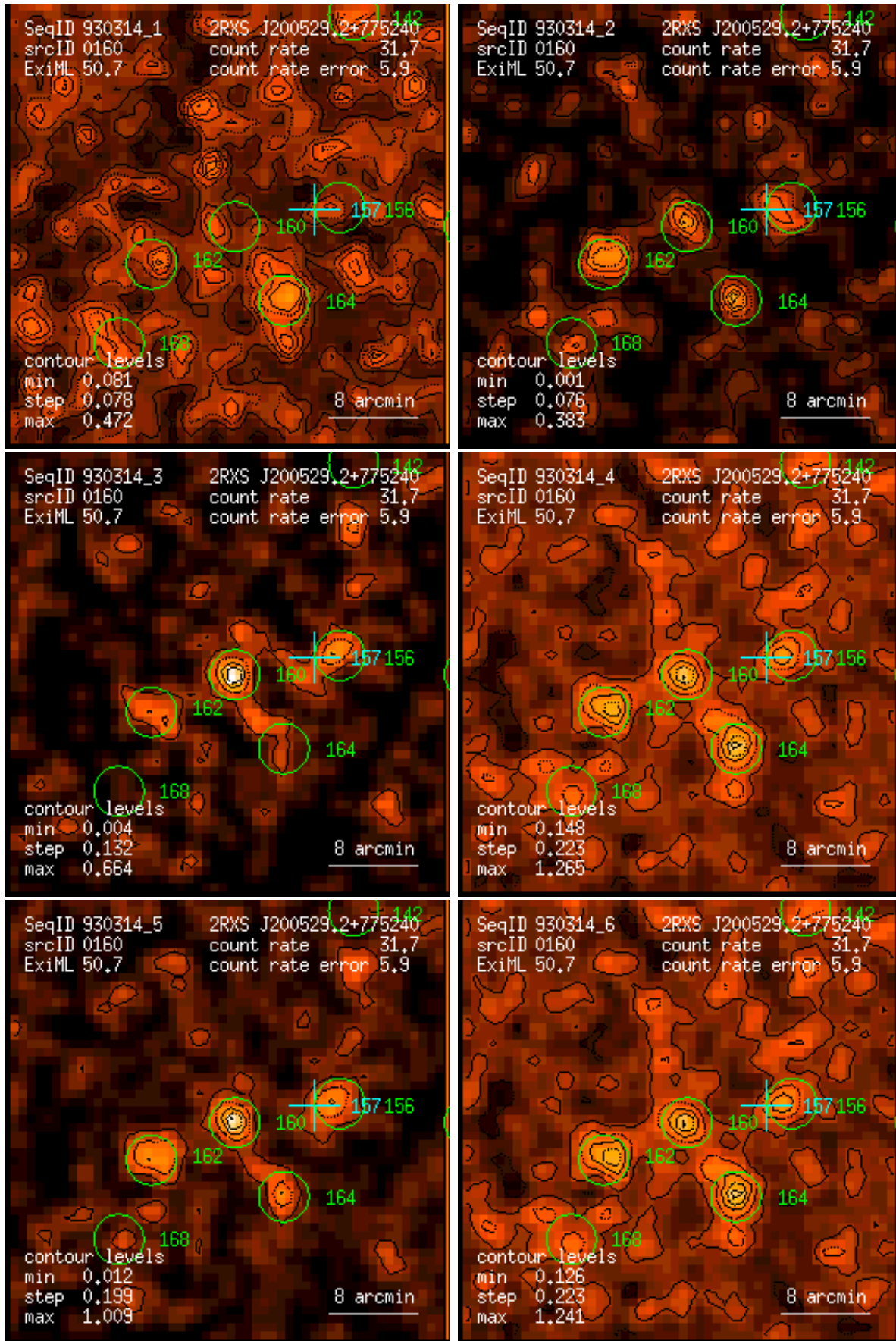
Figure 160: RASS 930314: detection 0160: band rate images, Gaussian filter: (1) PSPC channels 11 – 41, (2) 52 – 90, (3) 91 – 201, (4) 11 – 235, (5) 52 – 201, (6) 11 – 201. Broad band rates in counts/ks. Band rate contour levels in counts/ks/arcmin 2 .
