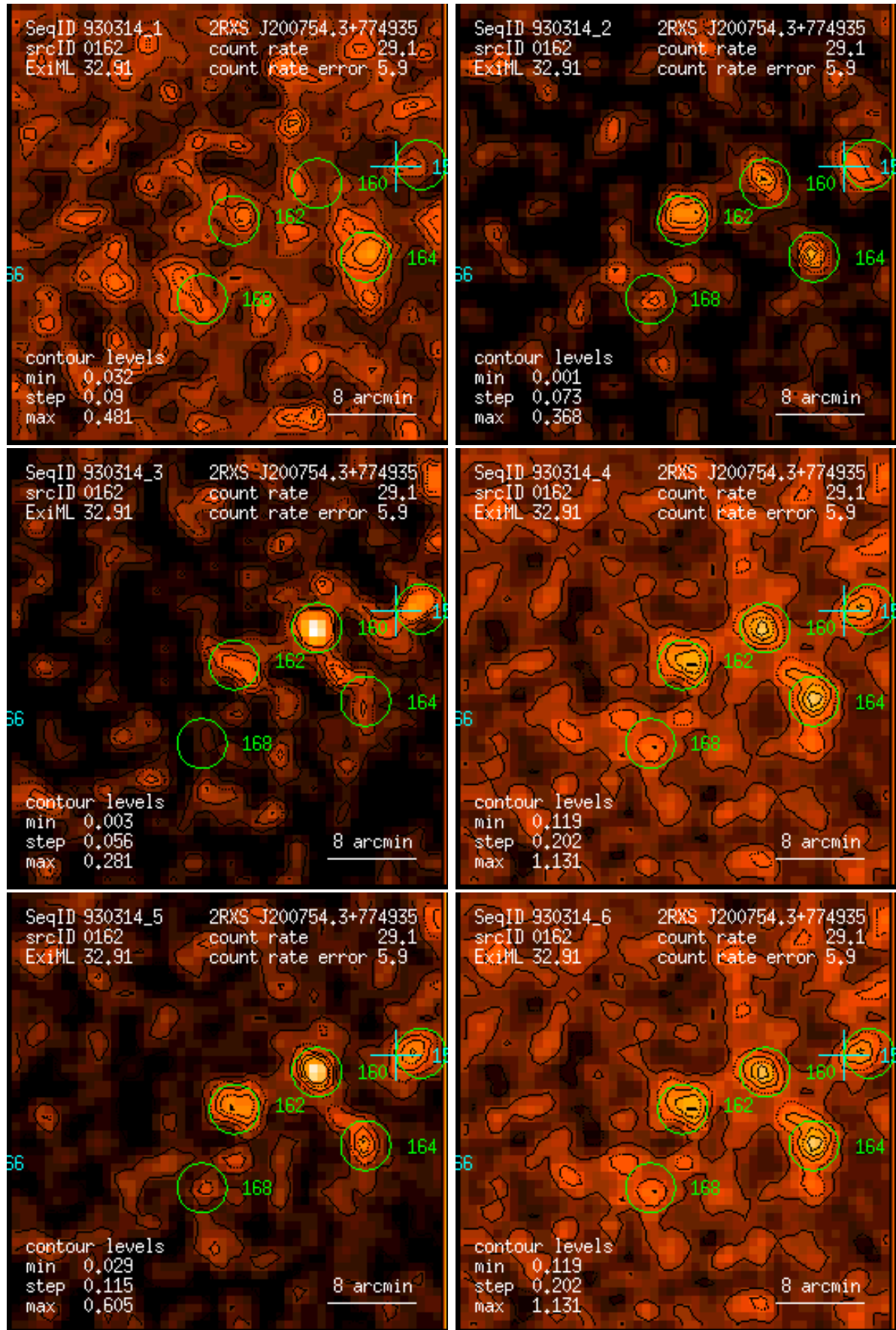
Figure 162: RASS 930314: detection 0162: band rate images, Gaussian filter: (1) PSPC channels 11 – 41, (2) 52 – 90, (3) 91 – 201, (4) 11 – 235, (5) 52 – 201, (6) 11 – 201. Broad band rates in counts/ks. Band rate contour levels in counts/ks/arcmin 2 .
