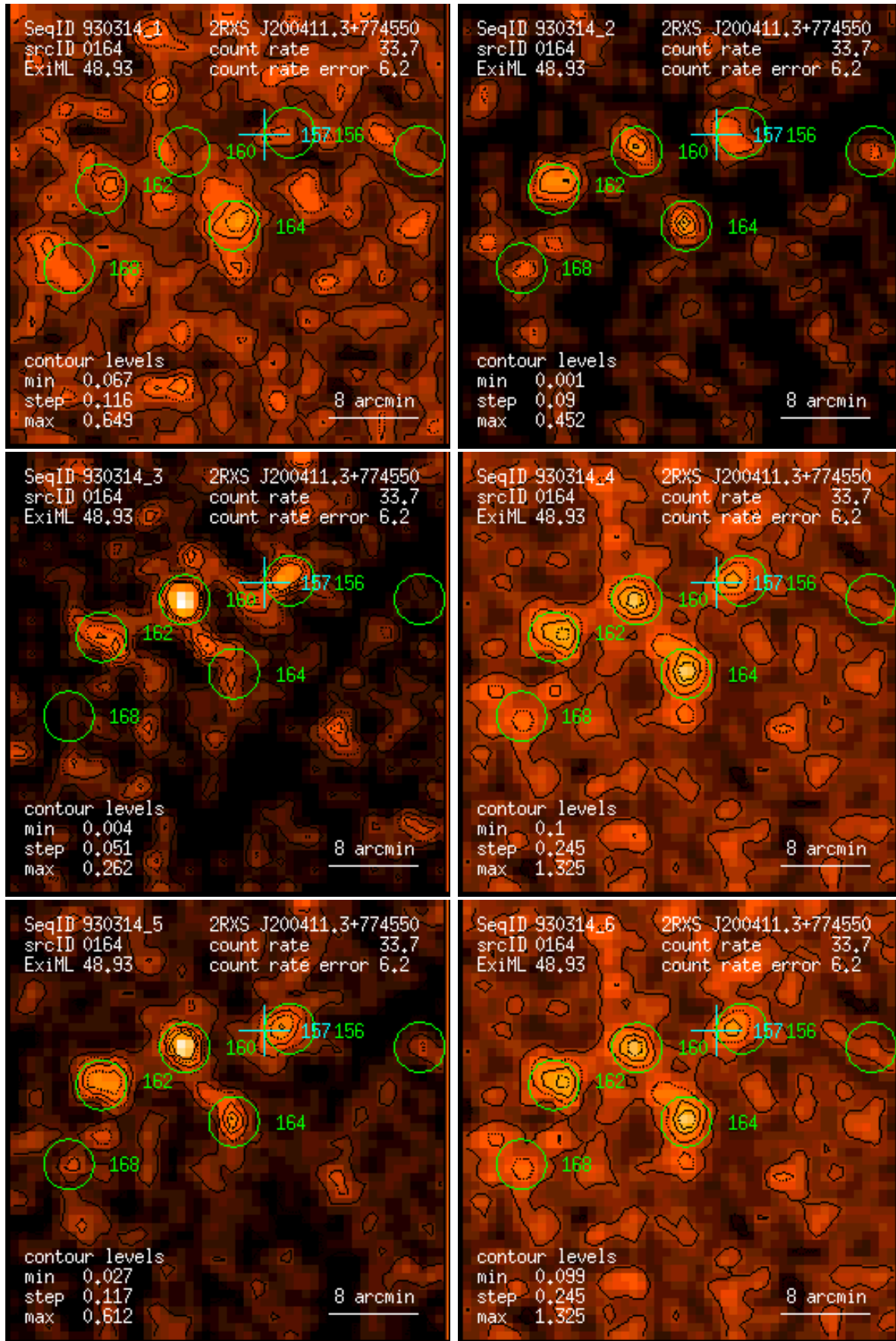
Figure 164: RASS 930314: detection 0164: band rate images, Gaussian filter: (1) PSPC channels 11 – 41, (2) 52 – 90, (3) 91 – 201, (4) 11 – 235, (5) 52 – 201, (6) 11 – 201. Broad band rates in counts/ks. Band rate contour levels in counts/ks/arcmin 2 .
