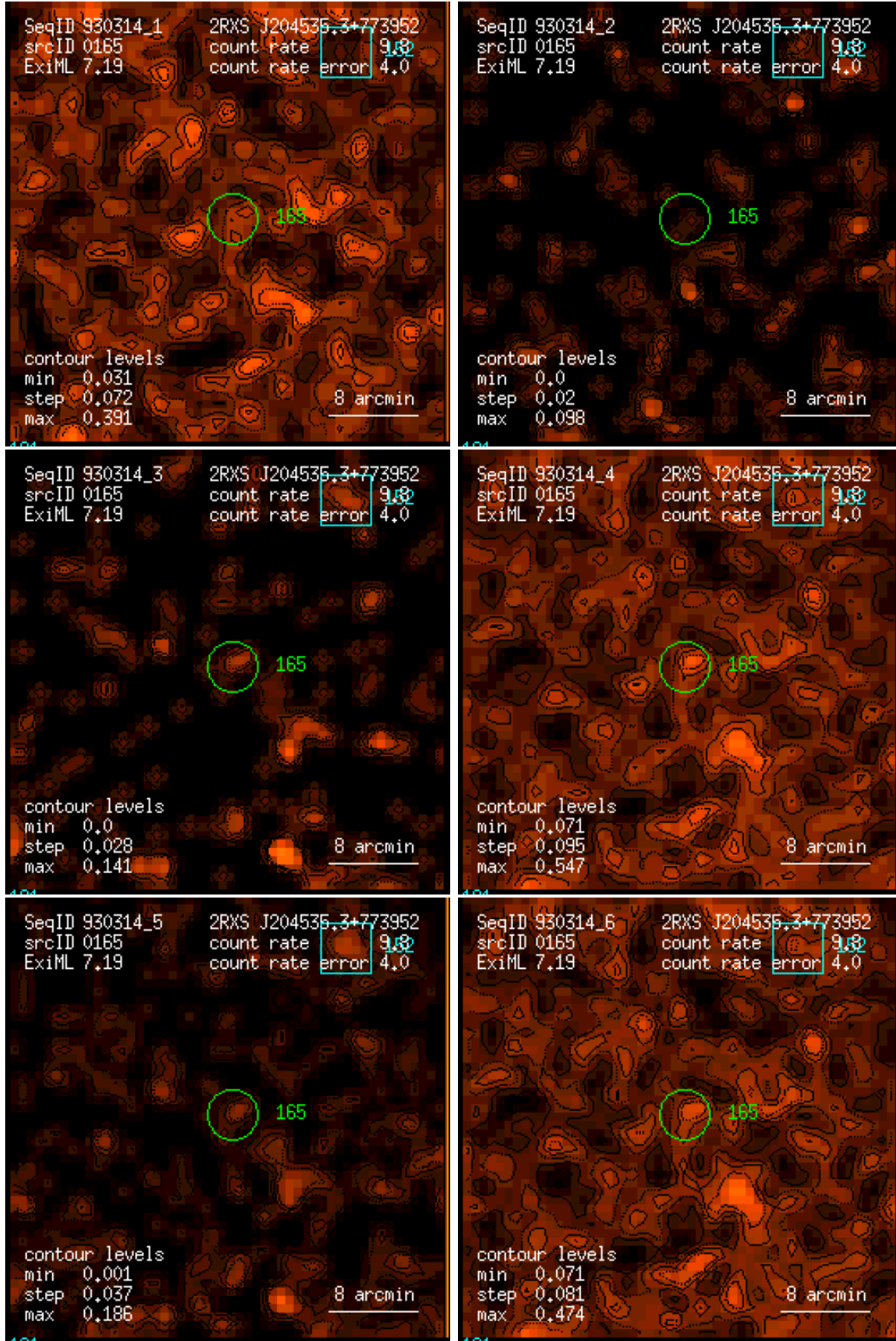
Figure 165: RASS 930314: detection 0165: band rate images, Gaussian filter: (1) PSPC channels 11 – 41, (2) 52 – 90, (3) 91 – 201, (4) 11 – 235, (5) 52 – 201, (6) 11 – 201. Broad band rates in counts/ks. Band rate contour levels in counts/ks/arcmin 2 .
