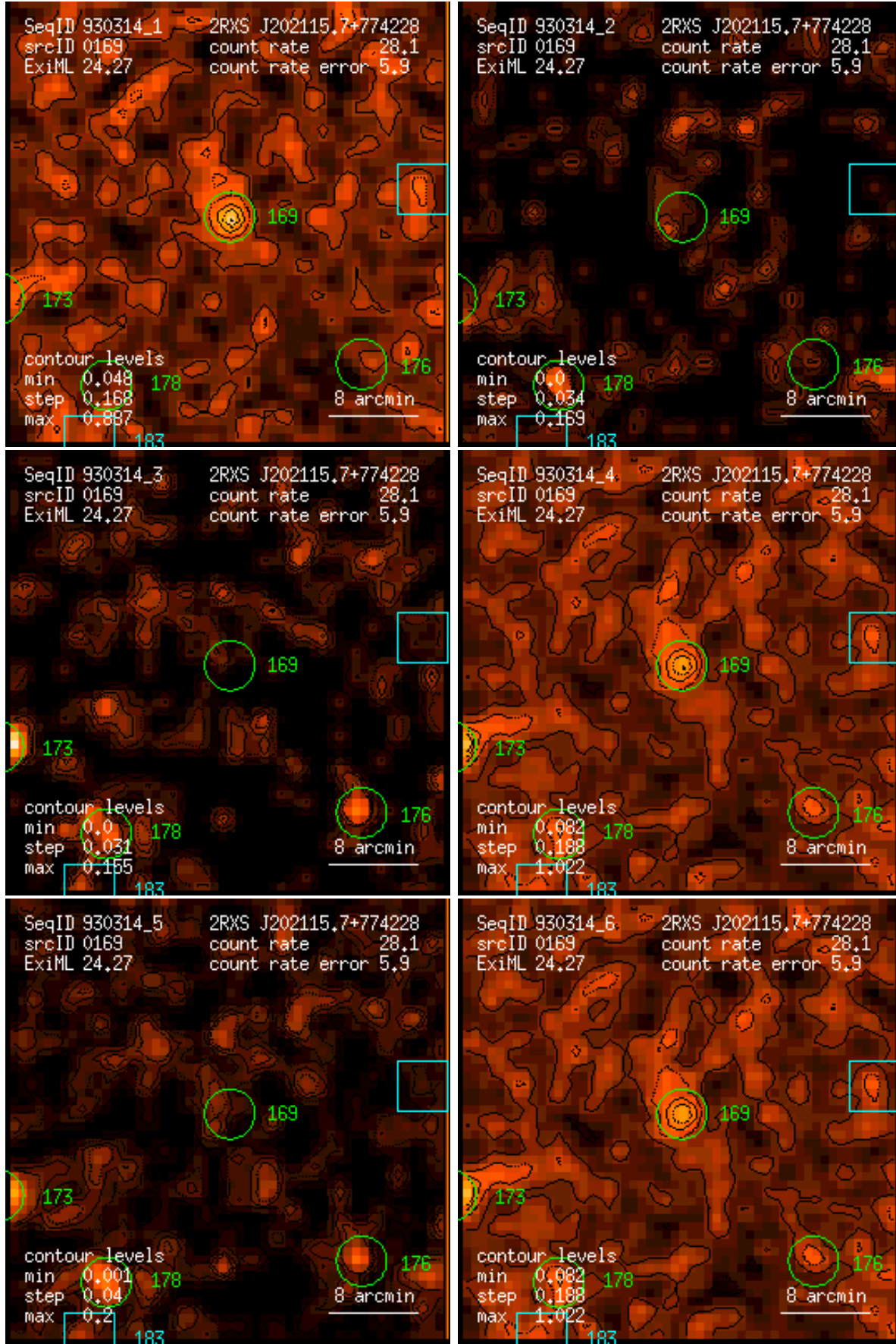
Figure 169: RASS 930314: detection 0169: band rate images, Gaussian filter: (1) PSPC channels 11 – 41, (2) 52 – 90, (3) 91 – 201, (4) 11 – 235, (5) 52 – 201, (6) 11 – 201. Broad band rates in counts/ks. Band rate contour levels in counts/ks/arcmin 2 .
