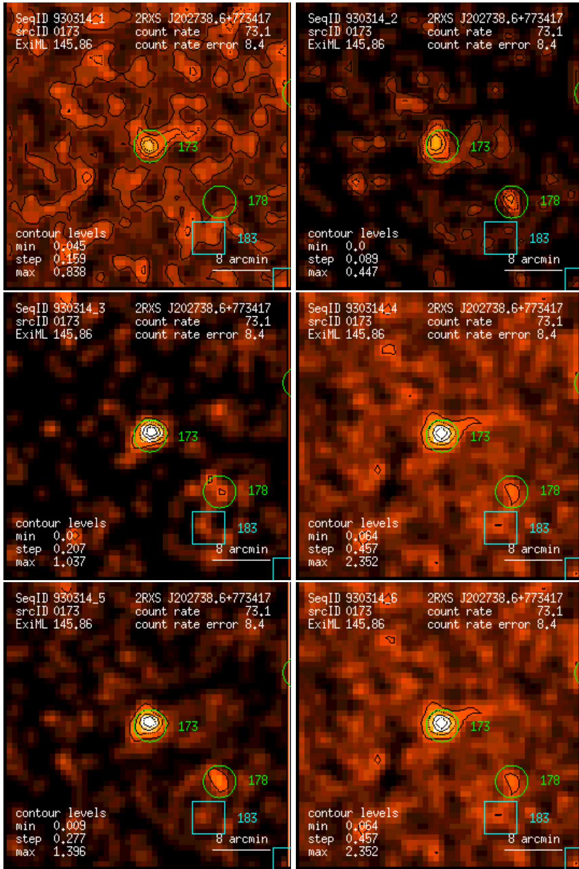
Figure 173: RASS 930314: detection 0173: band rate images, Gaussian filter: (1) PSPC channels 11 – 41, (2) 52 – 90, (3) 91 – 201, (4) 11 – 235, (5) 52 – 201, (6) 11 – 201. Broad band rates in counts/ks. Band rate contour levels in counts/ks/arcmin 2 .
