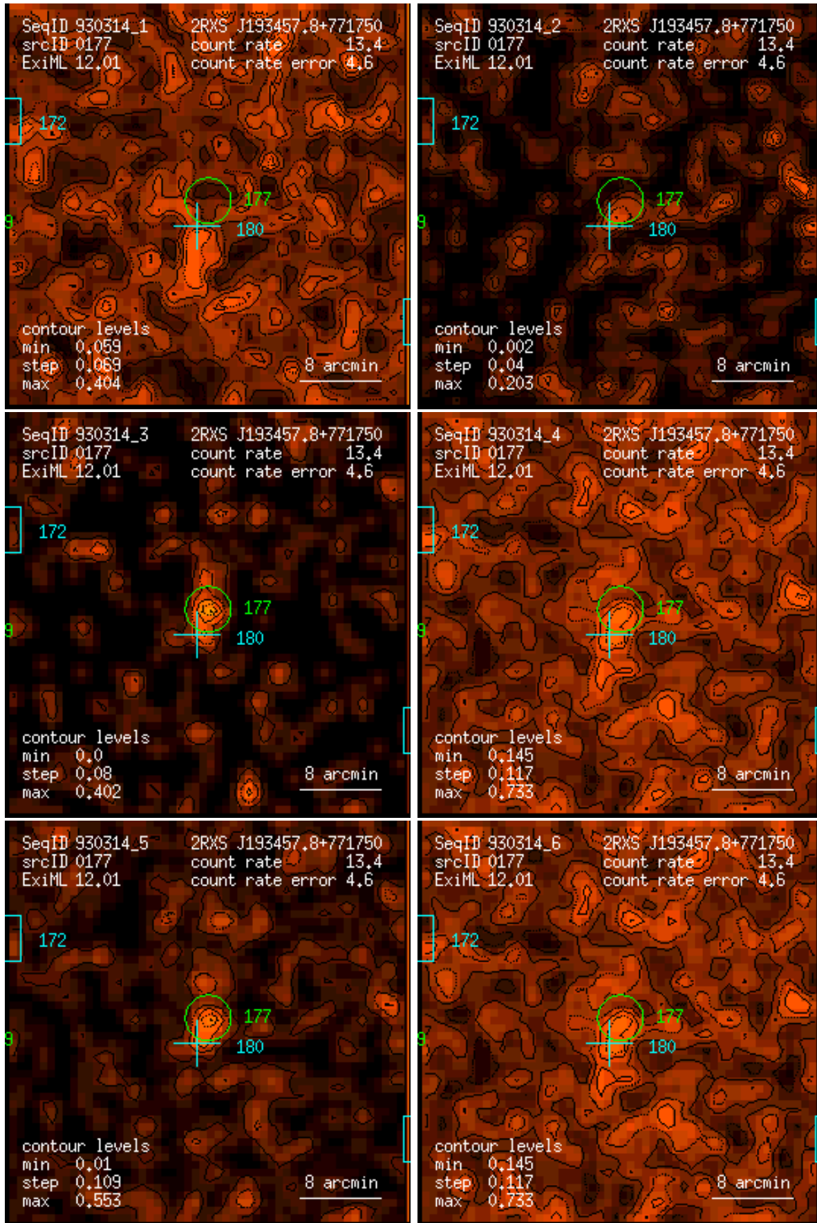
Figure 177: RASS 930314: detection 0177: band rate images, Gaussian filter: (1) PSPC channels 11 – 41, (2) 52 – 90, (3) 91 – 201, (4) 11 – 235, (5) 52 – 201, (6) 11 – 201. Broad band rates in counts/ks. Band rate contour levels in counts/ks/arcmin 2 .
