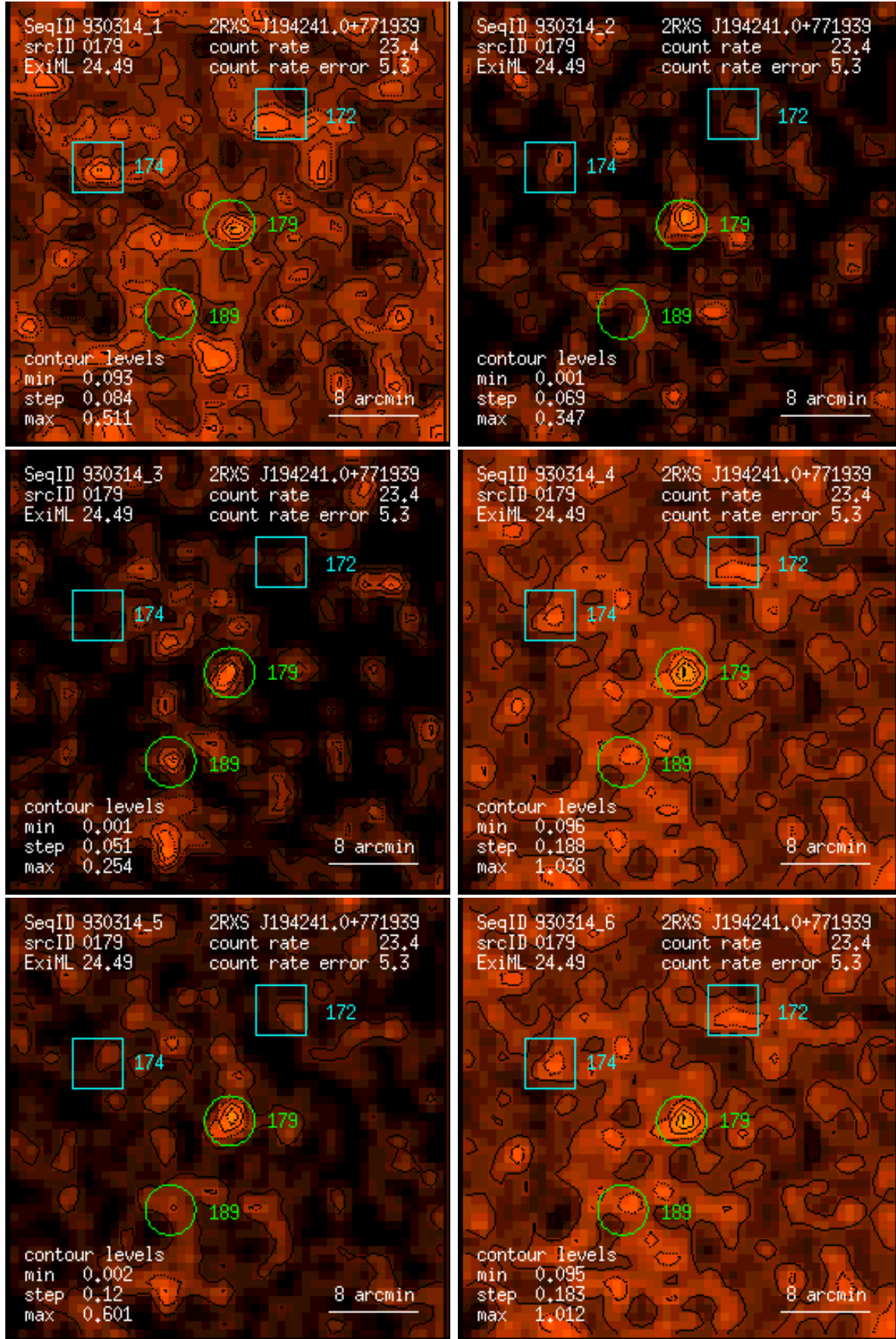
Figure 179: RASS 930314: detection 0179: band rate images, Gaussian filter: (1) PSPC channels 11 – 41, (2) 52 – 90, (3) 91 – 201, (4) 11 – 235, (5) 52 – 201, (6) 11 – 201. Broad band rates in counts/ks. Band rate contour levels in counts/ks/arcmin 2 .
