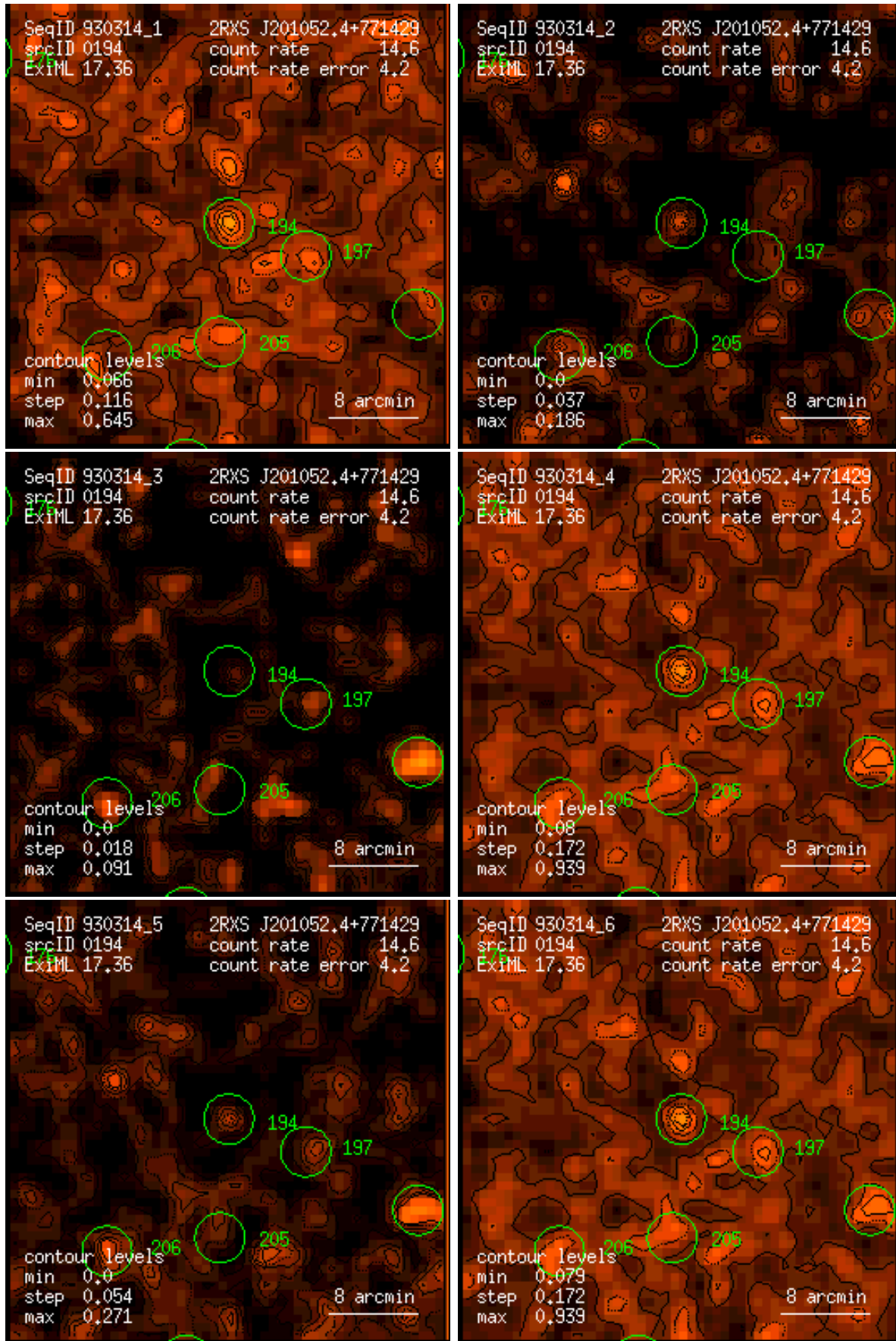
Figure 194: RASS 930314: detection 0194: band rate images, Gaussian filter: (1) PSPC channels 11 – 41, (2) 52 – 90, (3) 91 – 201, (4) 11 – 235, (5) 52 – 201, (6) 11 – 201. Broad band rates in counts/ks. Band rate contour levels in counts/ks/arcmin 2 .
