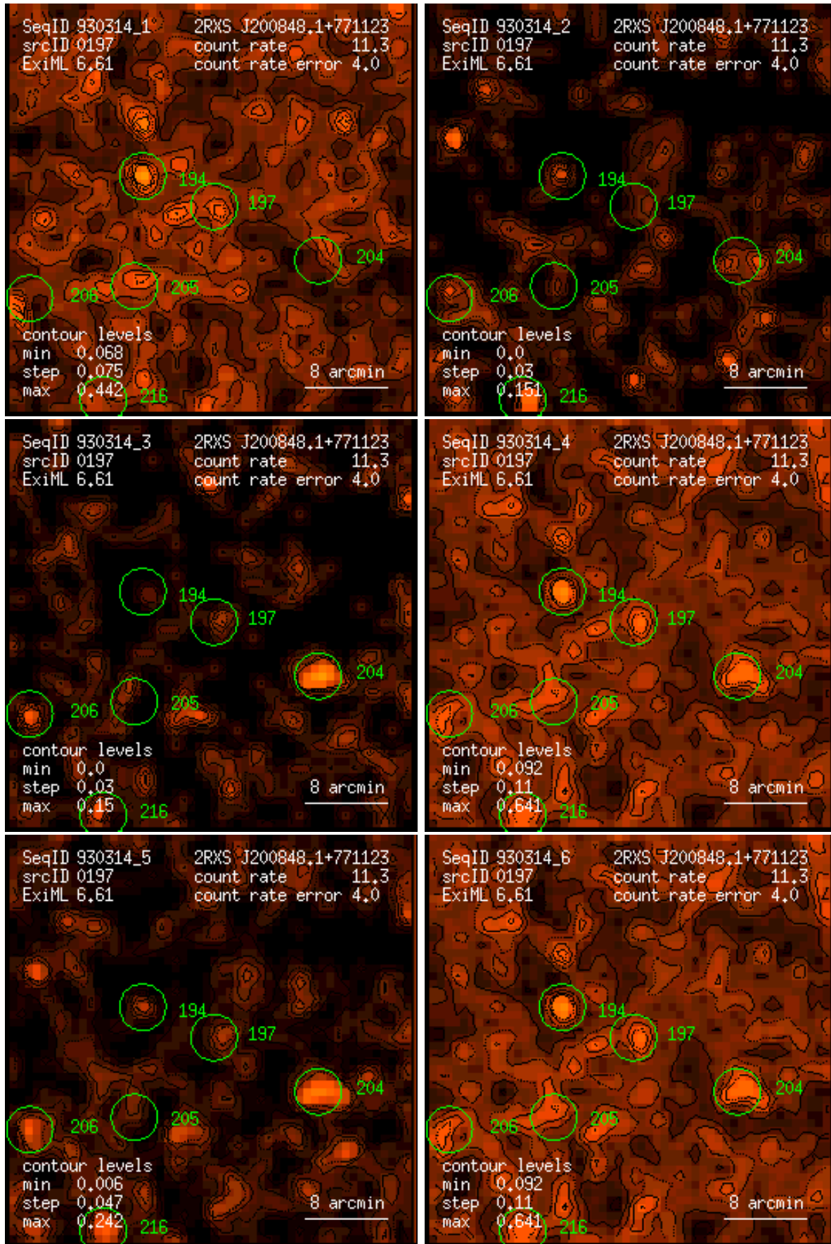
Figure 197: RASS 930314: detection 0197: band rate images, Gaussian filter: (1) PSPC channels 11 – 41, (2) 52 – 90, (3) 91 – 201, (4) 11 – 235, (5) 52 – 201, (6) 11 – 201. Broad band rates in counts/ks. Band rate contour levels in counts/ks/arcmin 2 .
