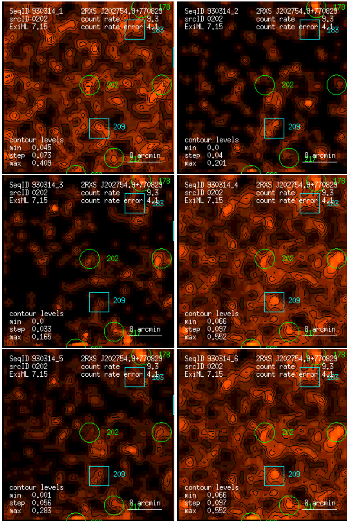
Figure 202: RASS 930314: detection 0202: band rate images, Gaussian filter: (1) PSPC channels 11 – 41, (2) 52 – 90, (3) 91 – 201, (4) 11 – 235, (5) 52 – 201, (6) 11 – 201. Broad band rates in counts/ks. Band rate contour levels in counts/ks/arcmin 2 .
