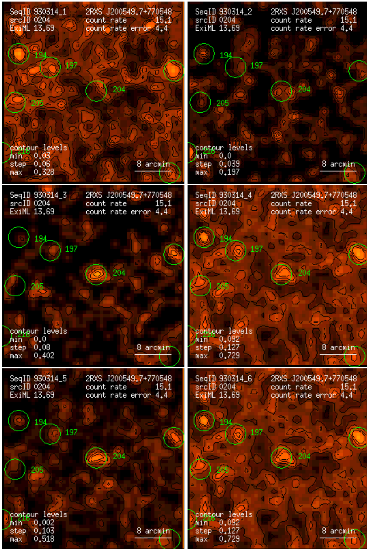
Figure 204: RASS 930314: detection 0204: band rate images, Gaussian filter: (1) PSPC channels 11 – 41, (2) 52 – 90, (3) 91 – 201, (4) 11 – 235, (5) 52 – 201, (6) 11 – 201. Broad band rates in counts/ks. Band rate contour levels in counts/ks/arcmin 2 .
