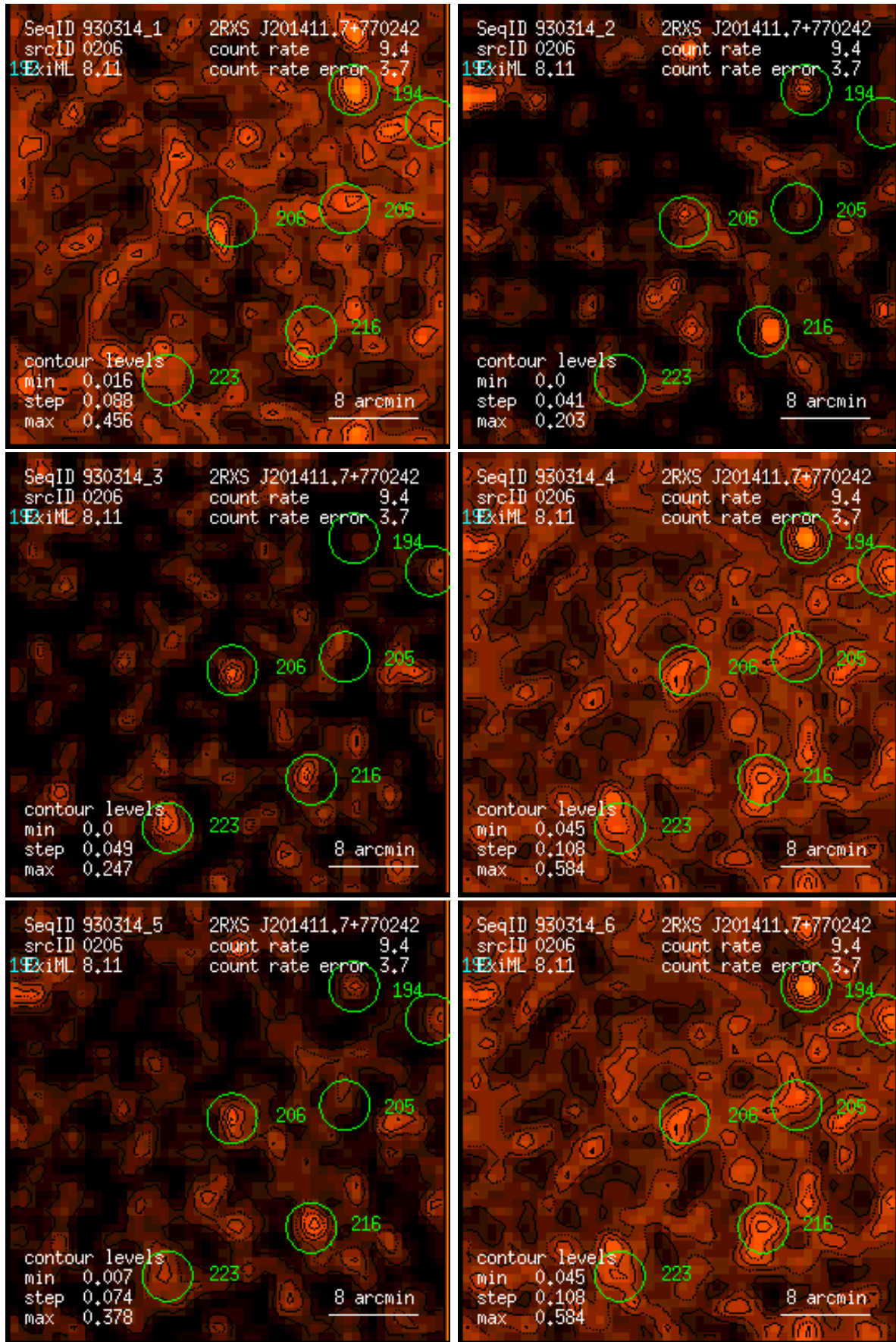
Figure 206: RASS 930314: detection 0206: band rate images, Gaussian filter: (1) PSPC channels 11 – 41, (2) 52 – 90, (3) 91 – 201, (4) 11 – 235, (5) 52 – 201, (6) 11 – 201. Broad band rates in counts/ks. Band rate contour levels in counts/ks/arcmin 2 .
