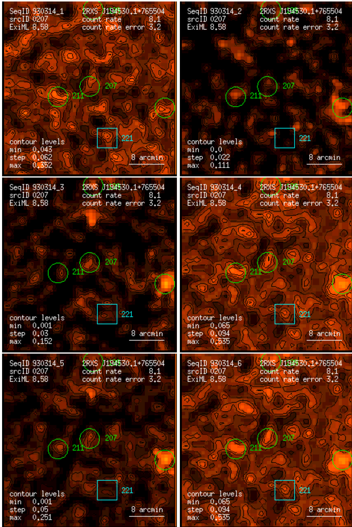
Figure 207: RASS 930314: detection 0207: band rate images, Gaussian filter: (1) PSPC channels 11 – 41, (2) 52 – 90, (3) 91 – 201, (4) 11 – 235, (5) 52 – 201, (6) 11 – 201. Broad band rates in counts/ks. Band rate contour levels in counts/ks/arcmin 2 .
