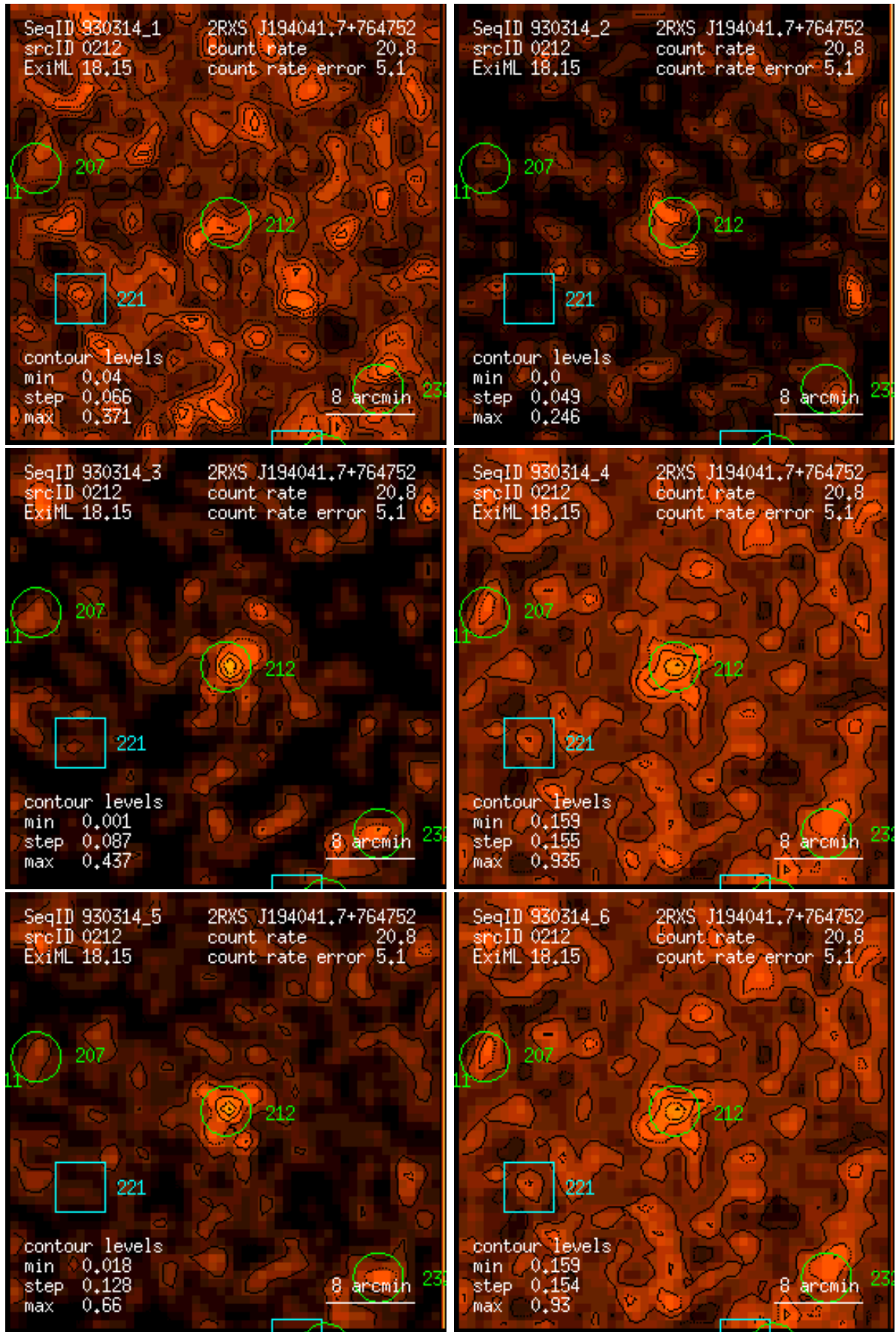
Figure 212: RASS 930314: detection 0212: band rate images, Gaussian filter: (1) PSPC channels 11 – 41, (2) 52 – 90, (3) 91 – 201, (4) 11 – 235, (5) 52 – 201, (6) 11 – 201. Broad band rates in counts/ks. Band rate contour levels in counts/ks/arcmin 2 .
