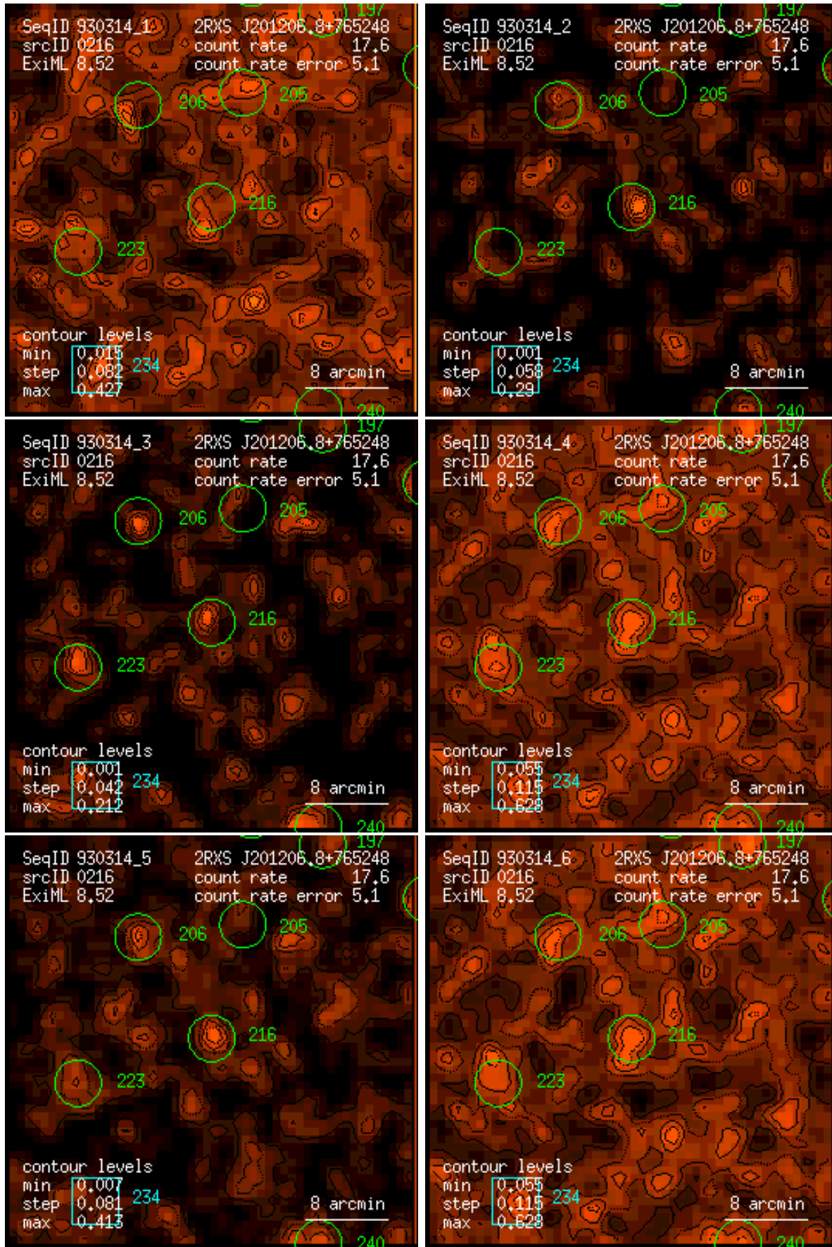
Figure 216: RASS 930314: detection 0216: band rate images, Gaussian filter: (1) PSPC channels 11 – 41, (2) 52 – 90, (3) 91 – 201, (4) 11 – 235, (5) 52 – 201, (6) 11 – 201. Broad band rates in counts/ks. Band rate contour levels in counts/ks/arcmin 2 .
