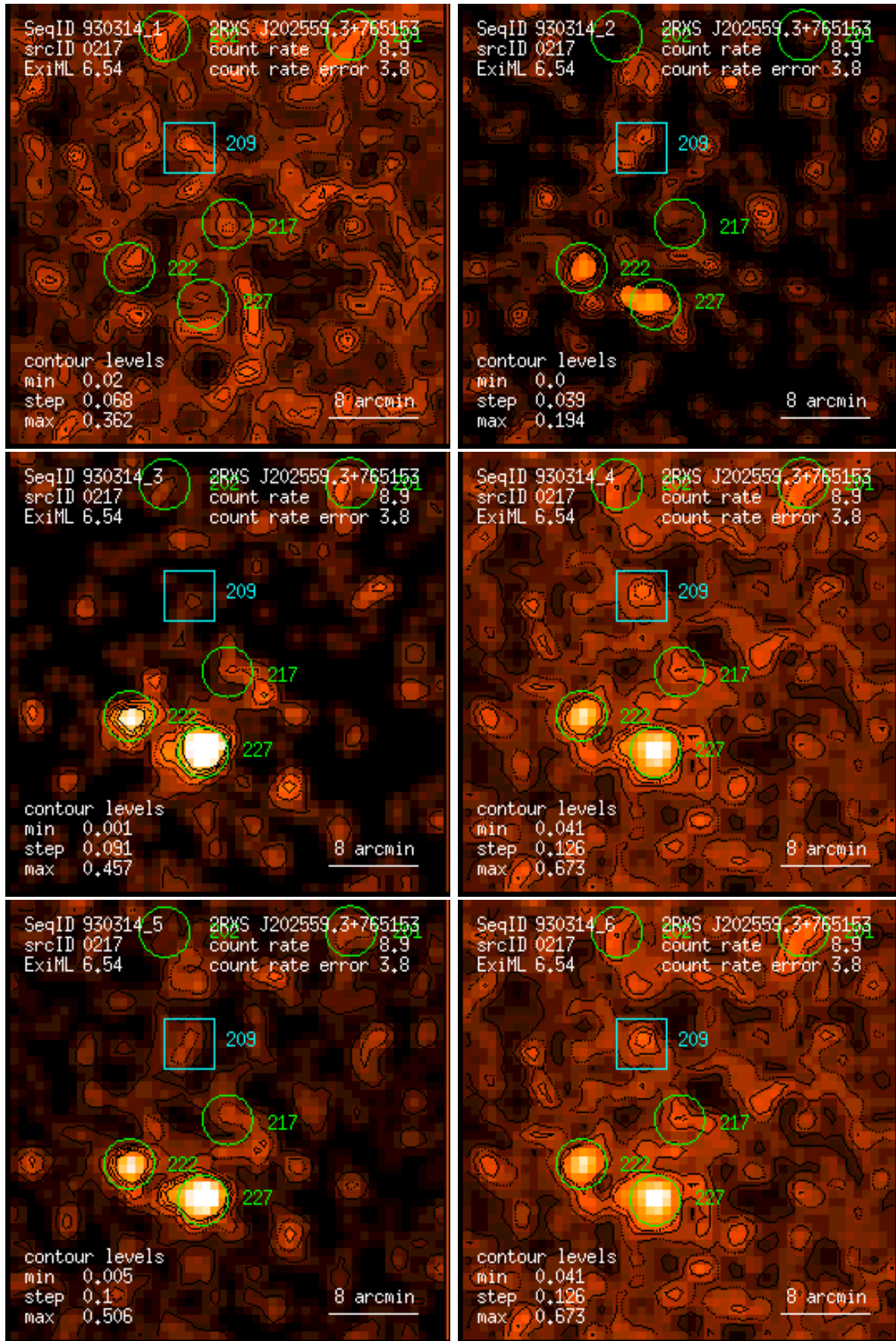
Figure 217: RASS 930314: detection 0217: band rate images, Gaussian filter: (1) PSPC channels 11 – 41, (2) 52 – 90, (3) 91 – 201, (4) 11 – 235, (5) 52 – 201, (6) 11 – 201. Broad band rates in counts/ks. Band rate contour levels in counts/ks/arcmin 2 .
