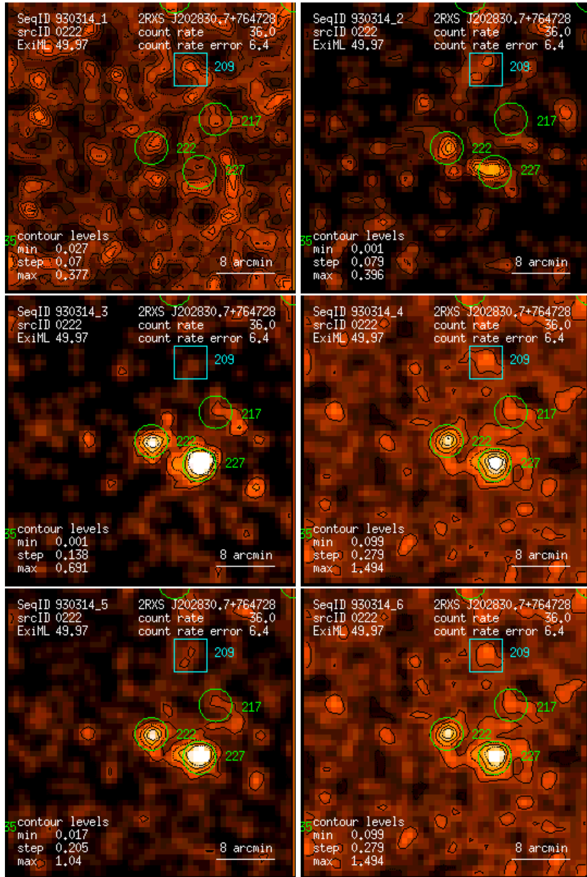
Figure 222: RASS 930314: detection 0222: band rate images, Gaussian filter: (1) PSPC channels 11 – 41, (2) 52 – 90, (3) 91 – 201, (4) 11 – 235, (5) 52 – 201, (6) 11 – 201. Broad band rates in counts/ks. Band rate contour levels in counts/ks/arcmin 2 .
